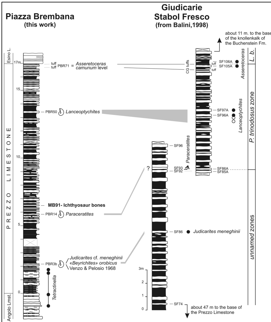
Fig. 4 - Ammonoid levels at the Piazza Brembana section and their correlation with the Stabol Fresco section in Giudicarie. The best ammonoid record for the Prezzo Limestone is from Stabol Fresco section (Balini 1992a, b, 1998) that is also the reference section for the formation (Gaetani 1970). Biostratigraphy is from Balini (1998): L.b.= Lardaroceras beds; CG tuffs= Contrada Gobbia tuffs. Black circle: occurrence in Stabol Fresco section; open circle: occurrence in the Adanà section, located about 400 m from Stabol Fresco section.
