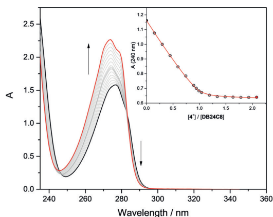
Figure 4. Absorption spectra of a 3.0 \times 10^{-4} M solution of DB24C8 in \text{CH}_2\text{Cl}_2 upon addition of 4^+ . The inset shows the absorption changes at 240 nm together with the fitted curve corresponding to a 1:1 binding model.
