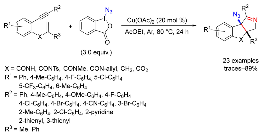
Scheme 43. Cu-catalyzed azidation of 1,6- or 1,7-enynes.
