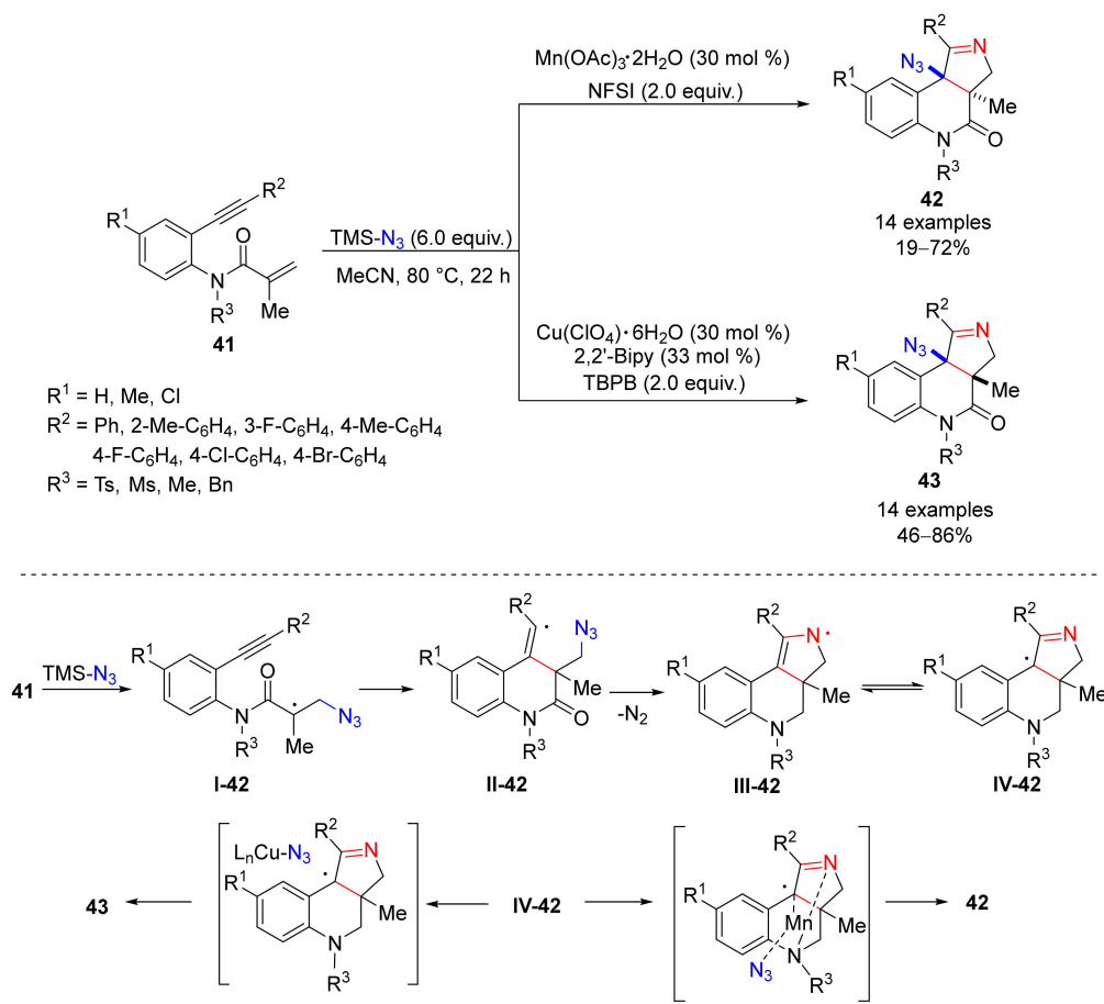
Scheme 42. Copper catalyzed azidation/cyclization of 1,7-enynes.
