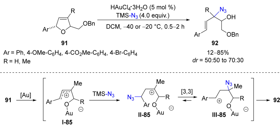
Scheme 85. Gold catalyzed ring-opening azidation.
