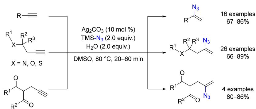
Scheme 82. Azidation of alkynes for the synthesis of azidovinyl-compounds.
