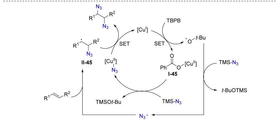
Scheme 45. Cu-catalyzed diazidation.
