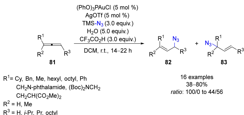
Scheme 78. Gold(I)-catalyzed azidation of allenes.
