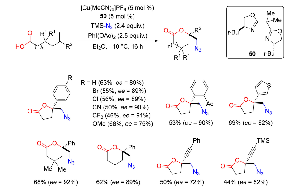
Scheme 54. Enantioselective Cu-catalyzed cyclization/azidation reactions of alkene-containing carboxylic acids.
