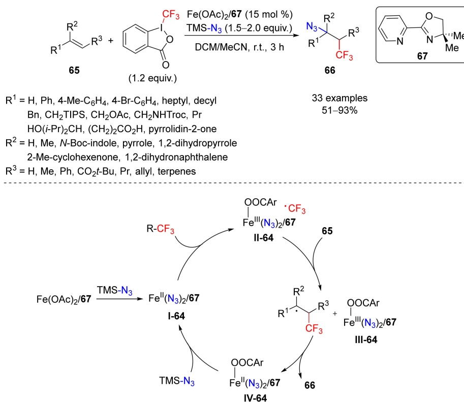
Scheme 64. Enantioselective azidotrifluoromethylation of olefins via iron catalysis.
