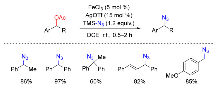
Scheme 6. Azidation via nucleophilic substitution of benzylic acetates.
