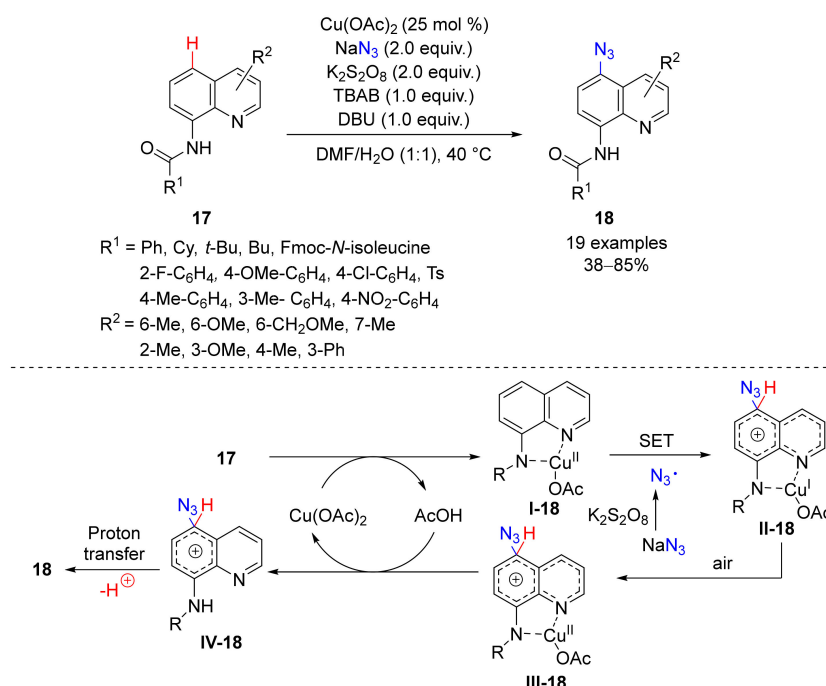
Scheme 18. C-H azidation of quinolines by Cu(OAc) 2 catalysis.
