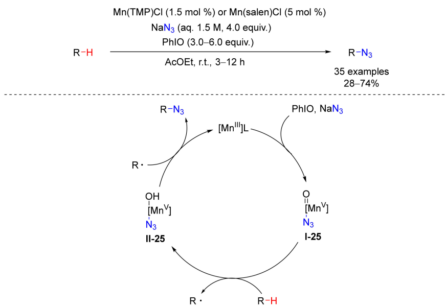
Scheme 25. Aliphatic C–H azidation procedure.
