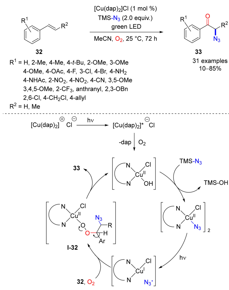
Scheme 32. Regio- and chemoselective oxyazidation of vinyl arenes.
