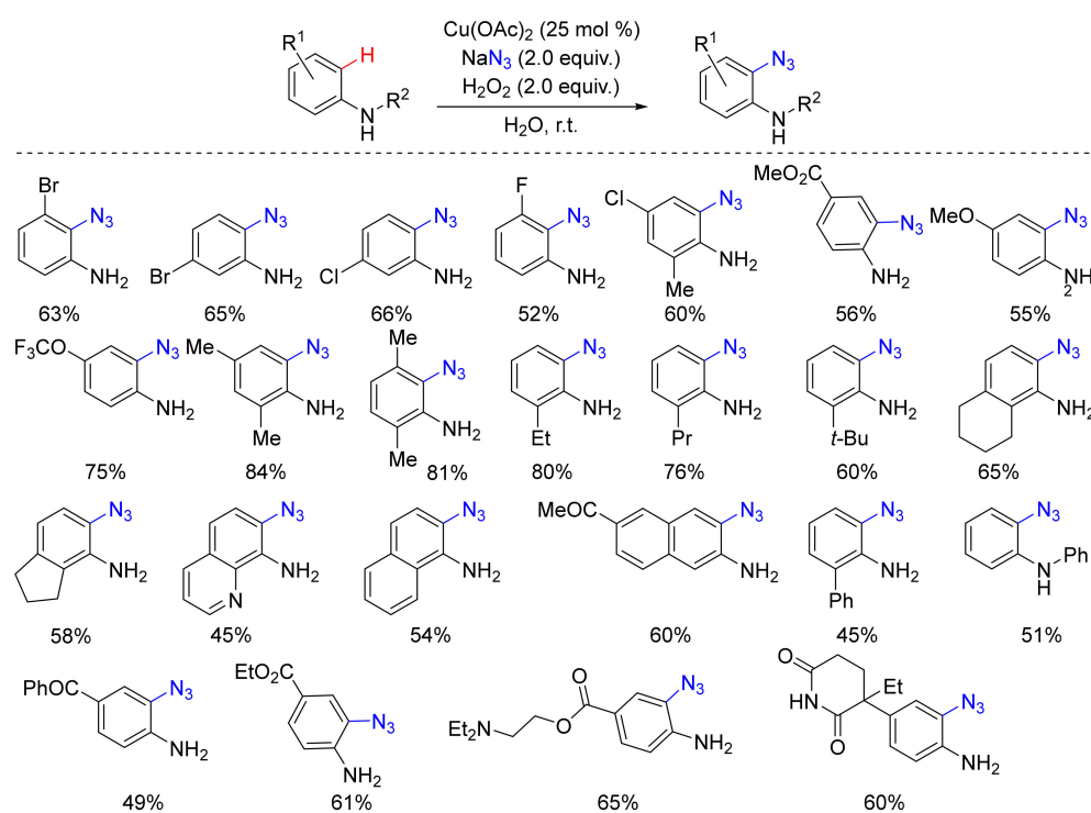
Scheme 16. Copper catalyzed C-H azidation of anilines.
