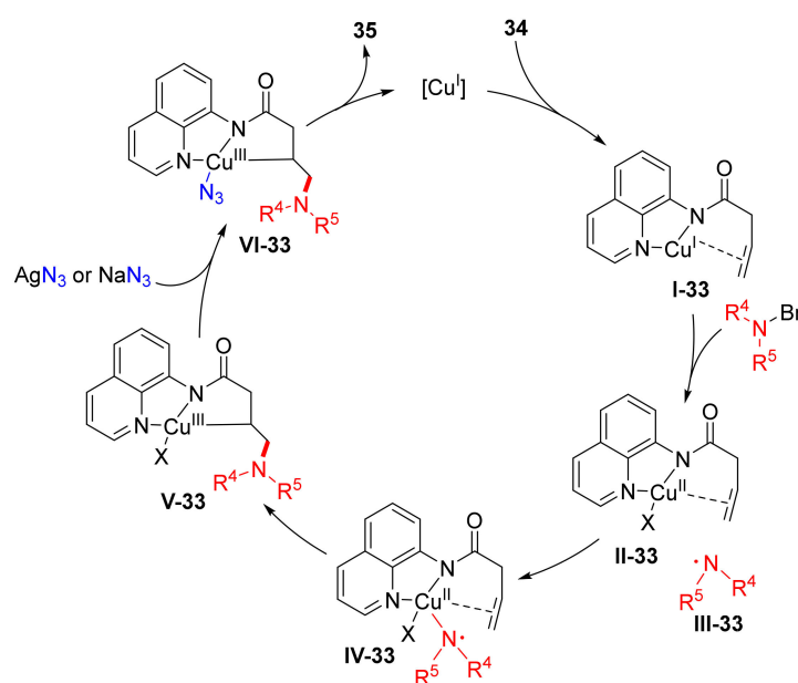
Scheme 33. Cu-catalyzed amination/azidation reaction.
