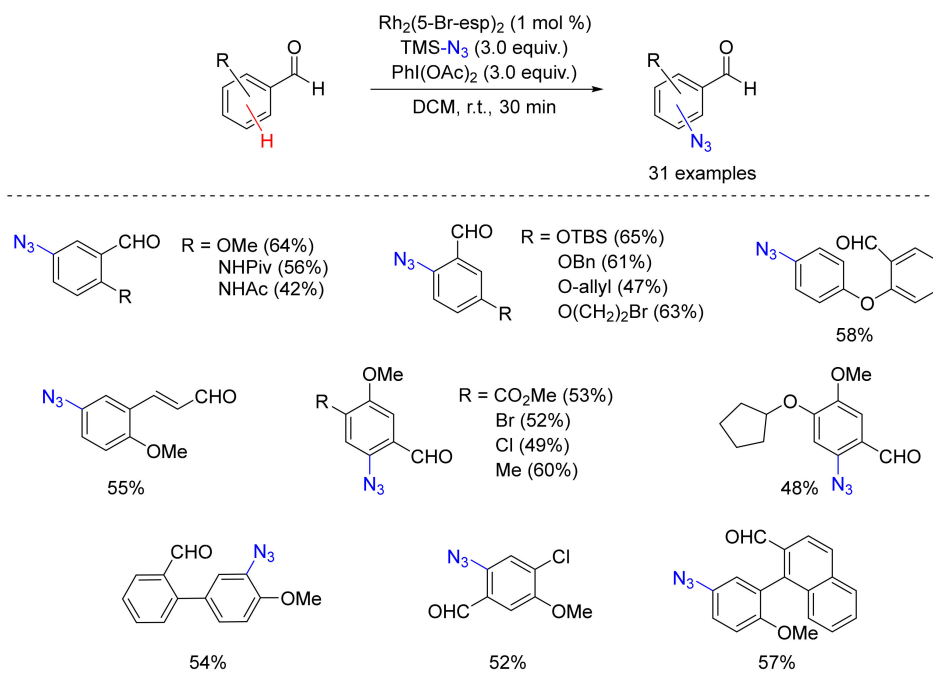
Scheme 24. Dirhodium(II) direct azidation of aromatic aldehydes.
