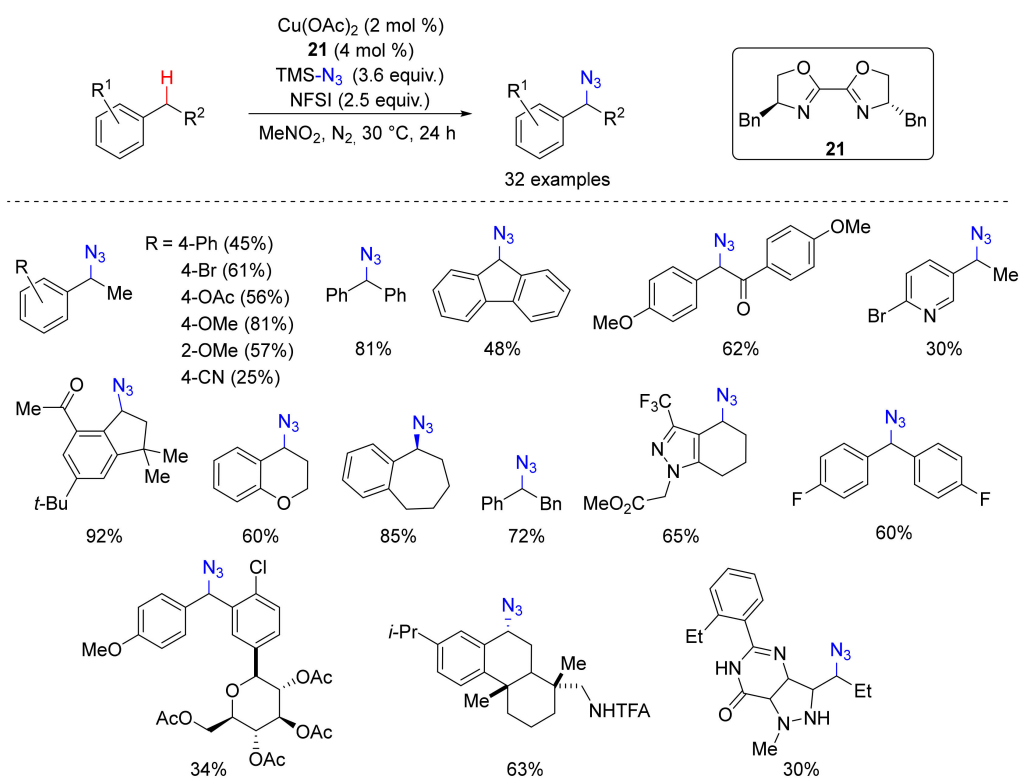
Scheme 20. Oxidative copper catalyzed C( sp 3 )-H azidation.
