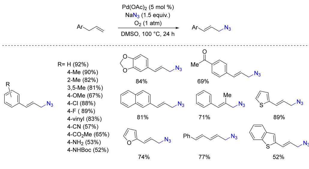
Scheme 75. Conversion of terminal alkenes into allyl azides in Pd(II)-catalyzed oxidative conditions.
