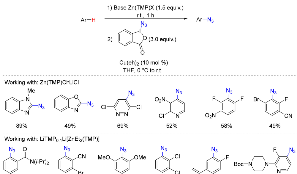
Scheme 21. Zinc-based assisted copper catalyzed azidation of arenes.
