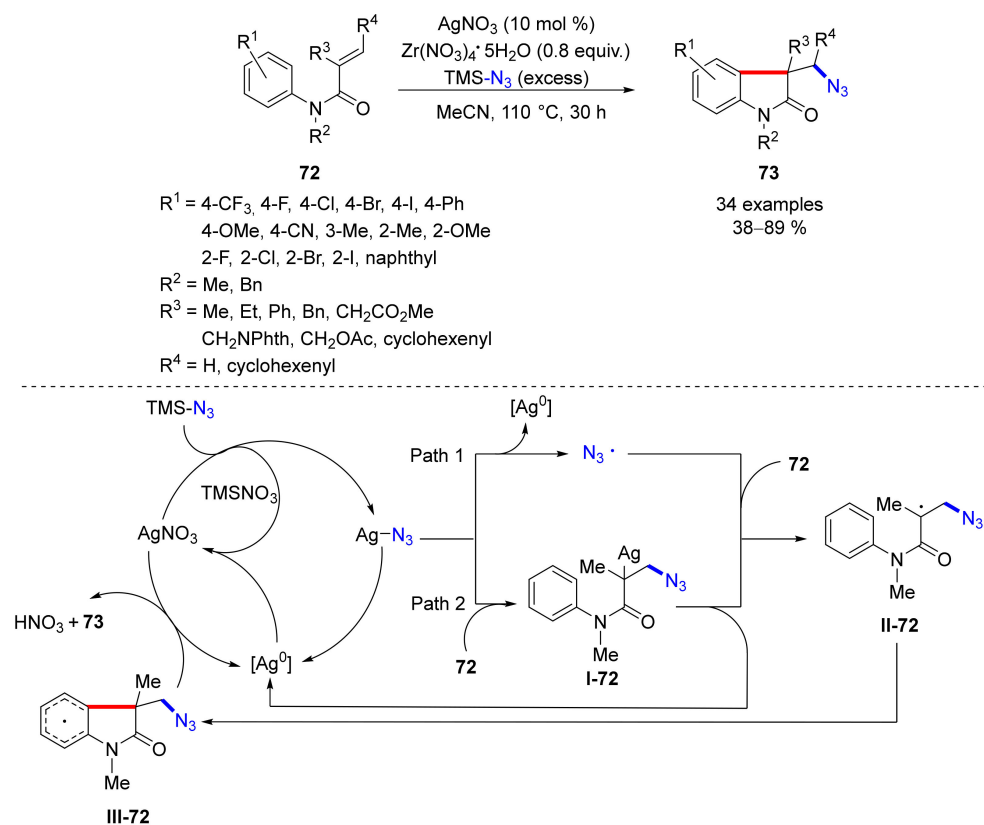
Scheme 72. Radical-silver catalyzed procedure of arylacrylamides.
