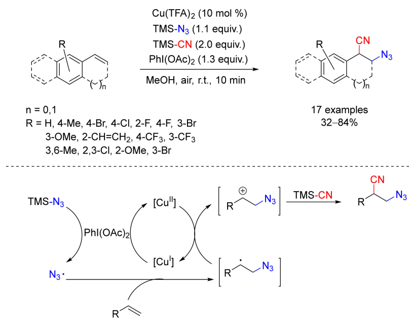
Scheme 74. Copper catalyzed azidocyanation of alkenes.
