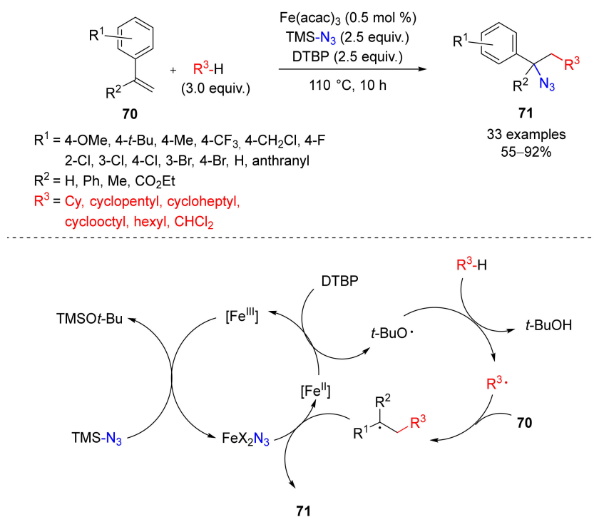
Scheme 70. Alkenes iron catalyzed carboazidation of styrenes.
