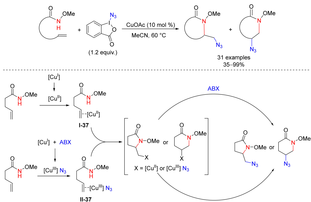
Scheme 37. Copper catalyzed aminoazidation of alkenes.
