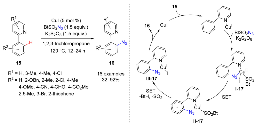
Scheme 17. Pyridine as directing group for the C-H azidation of arenes.
