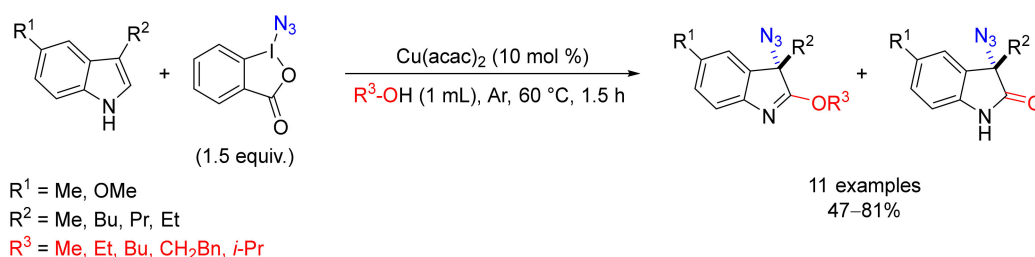
Scheme 52. Oxoazidation of indoles with 1-Azido-1,2-benziodoxol-3(1H)-one (ABX).
