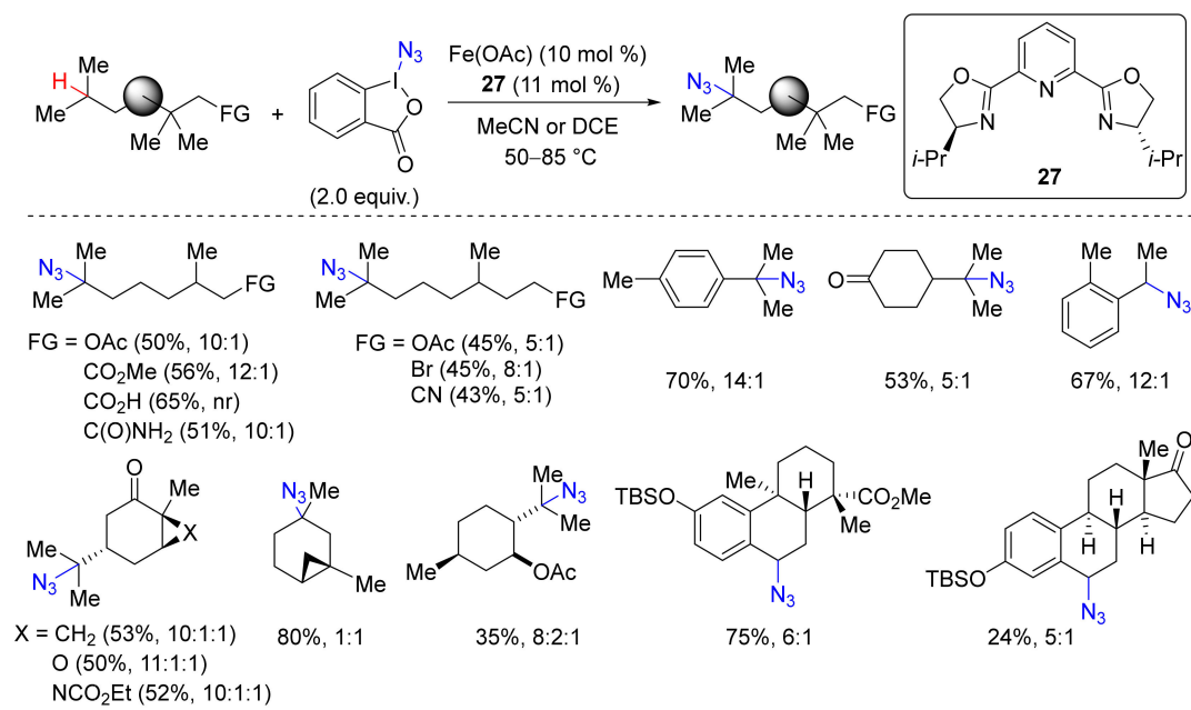
Scheme 27. Iron catalyzed azidation of unactivated tertiary C–H bond.
