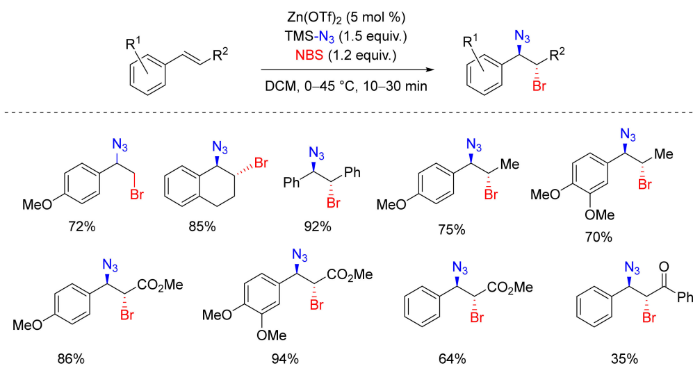
Scheme 68. Zn-catalyzed bromoazidation of alkenes.
