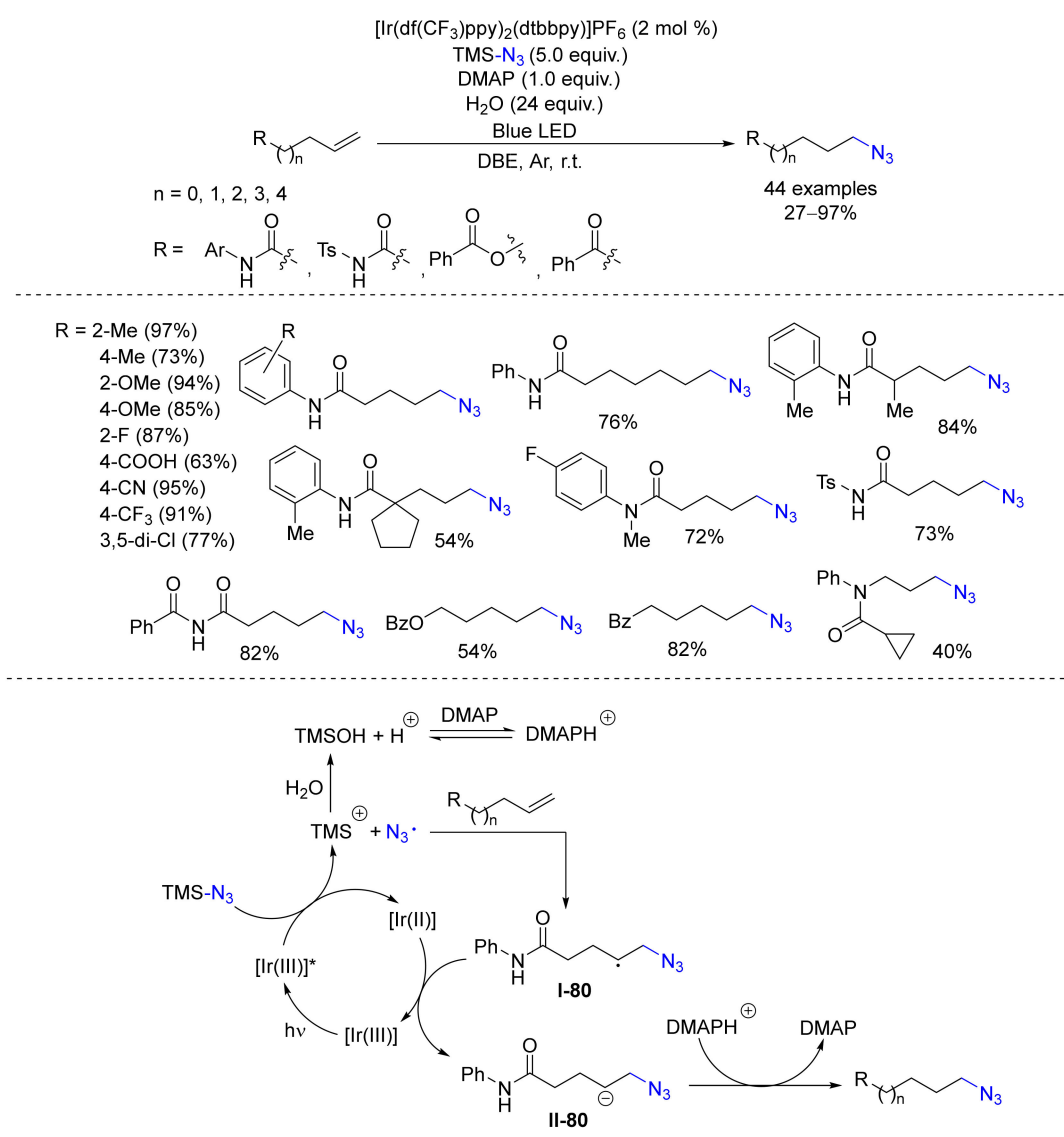
Scheme 80. Ir(III) catalyzed terminal alkenes hydroazidation.
