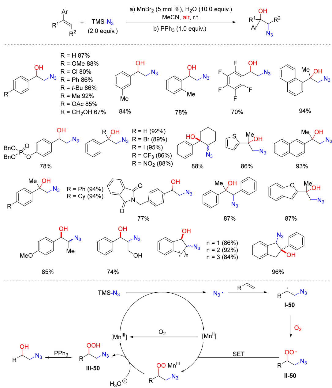
Scheme 50. Hydroxyazidation of terminal and internal styrenes.
