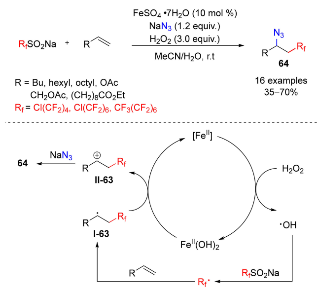
Scheme 63. Fenton reagent catalyzed radical carboazidation of alkenes.
