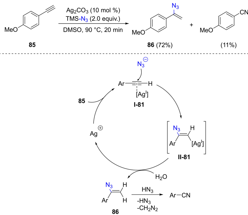
Scheme 81. Azidation of terminal alkynes for the formation of nitriles.
