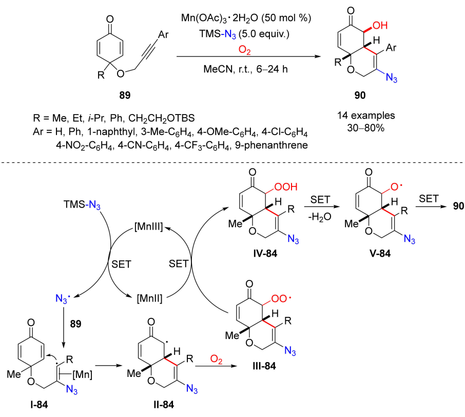
Scheme 84. Procedure for the synthesis of bicyclic azido alcohols.
