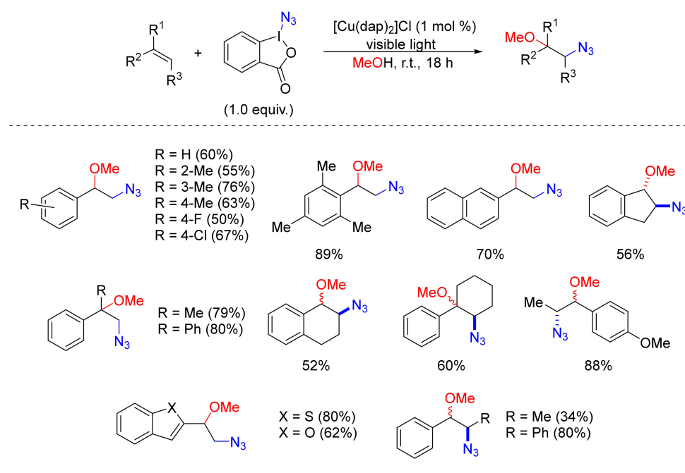
Scheme 51. Cu(I)-catalyzed methoxyazidation.
