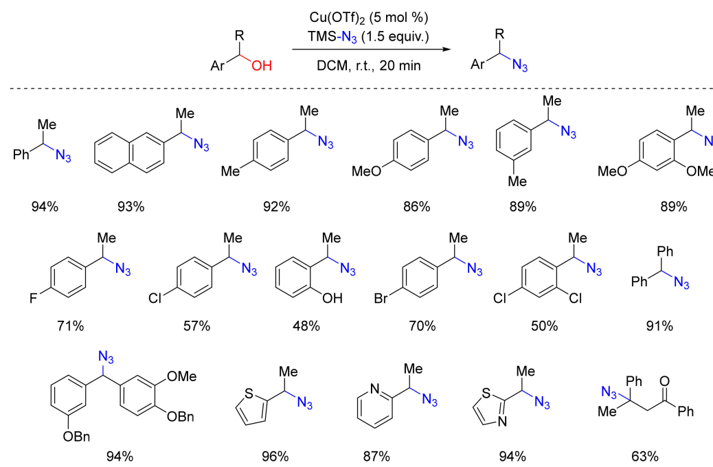
Scheme 10. Copper catalyzed conversion of benzyl alcohols into the corresponding azides.
