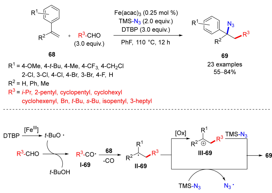
Scheme 69. Decarbonylative iron catalyzed carboazidation of styrenes.
