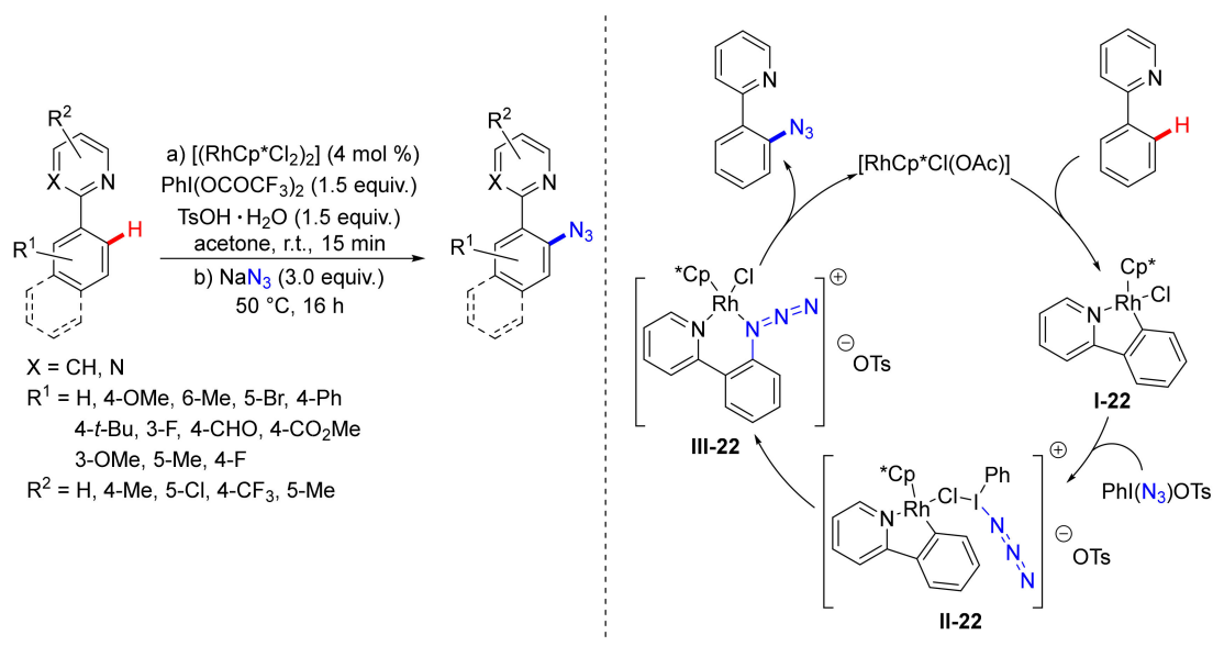
Scheme 22. Rh(III)-catalyzed C–H azidation of arenes.
