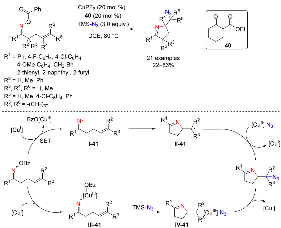
Scheme 41. Imination/azidation procedure.
