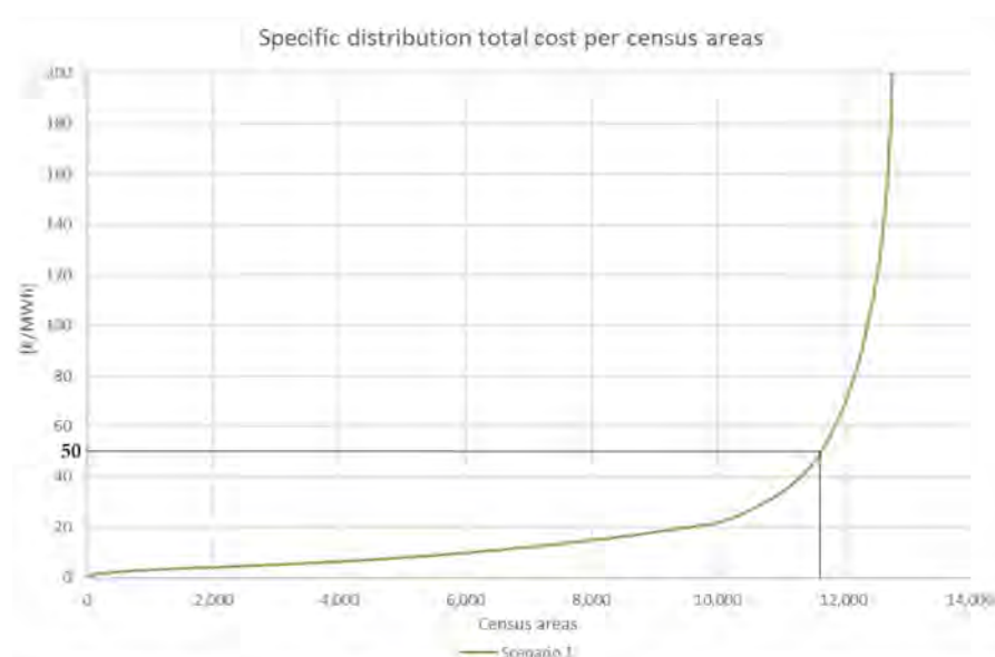
Figure 11. Specific distribution total cost per census area for scenario 1. Results representative of the reference methodology.
