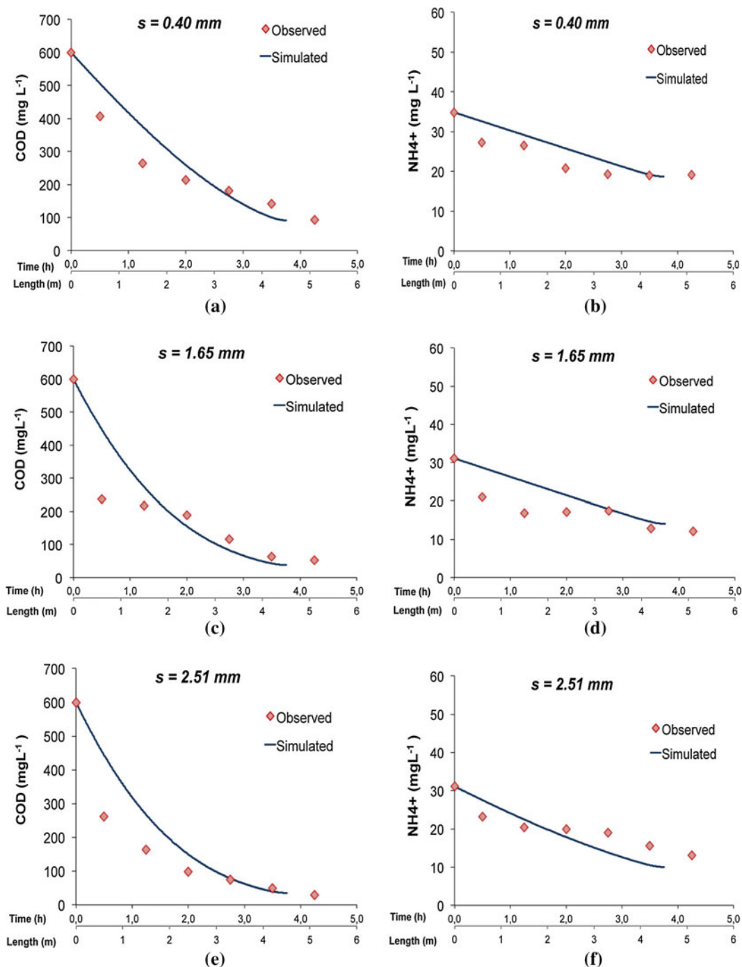
Fig. 5 Observed and simulated COD and NH 4 + concentration trend for different biofilm thickness
