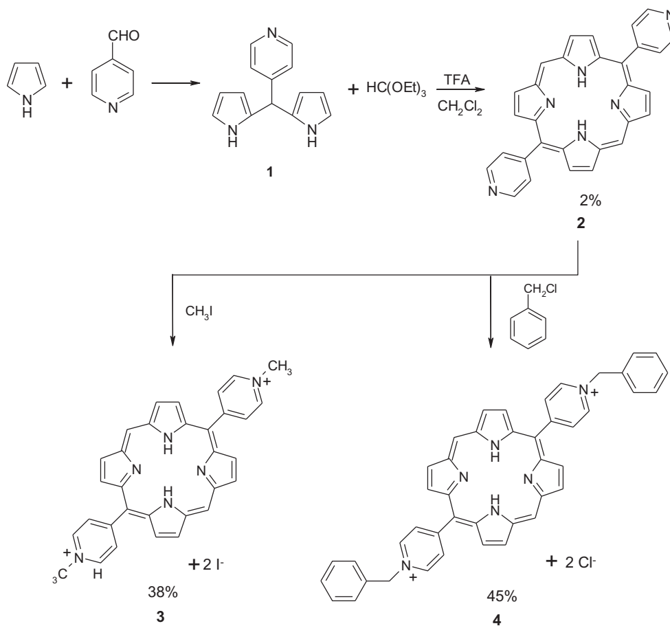
Scheme 1. Synthesis of the two cationic diarylporphyrins 3 and 4 .
