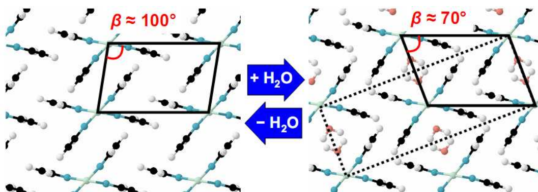
Figure 9. Left: view of the lattice structures of \beta -[Cu(pz) 2 ] n , 2 , down the (010) plane. Right: view of the lattice structure of [Cu(pz) 2 ·(H 2 O)] n , 3 , down the (001) plane. Solid lines show the monoclinic cells. The dashed line on the [Cu(pz) 2 ·(H 2 O)] n , 3 structure indicates the orthorhombic cell.
