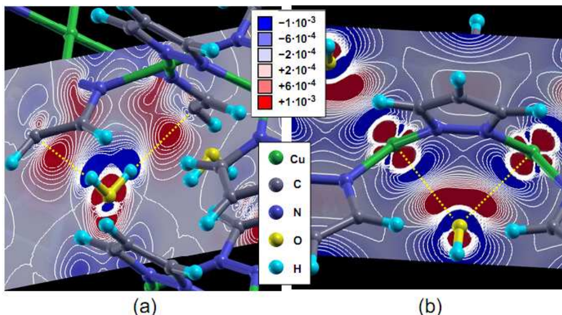
Figure 8. Electron difference density plots referring to the H 2 O - Cu(pz) 2 interaction (see text). Displayed sections are: (a) a (100) plane bisecting two pyrazolate rings which bridge the same Cu atoms; (b) a (001) plane passing through the Cu atoms of a polymer chain.
