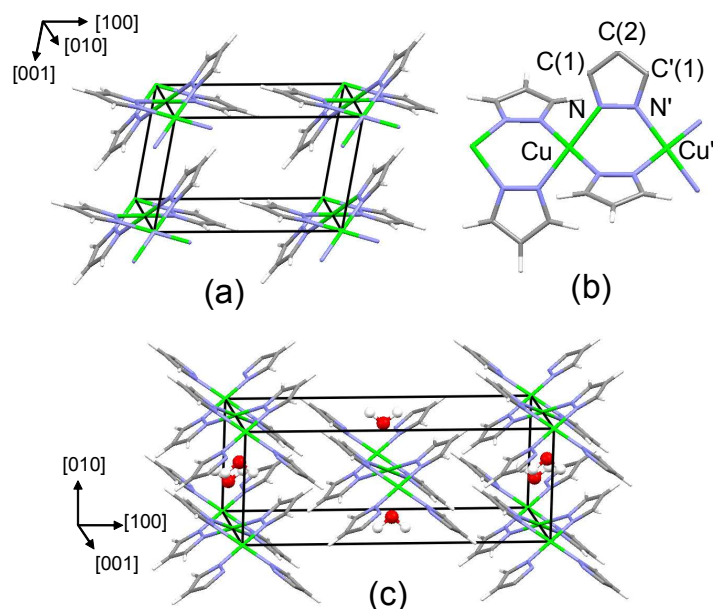
Figure 1. (a) Schematic drawings of: (a) \beta - [\text{Cu}(\text{pz})_2]_n ; (b) a portion of the \text{Cu}(\text{pz})_2 chain running along [010] ; (c) the unit cell of [\text{Cu}(\text{pz})_2 \cdot (\text{H}_2\text{O})]_n . The \text{H}_2\text{O} molecules, shown in a ball-and-stick representation, are in the equilibrium configuration as determined by the DFT calculations.
