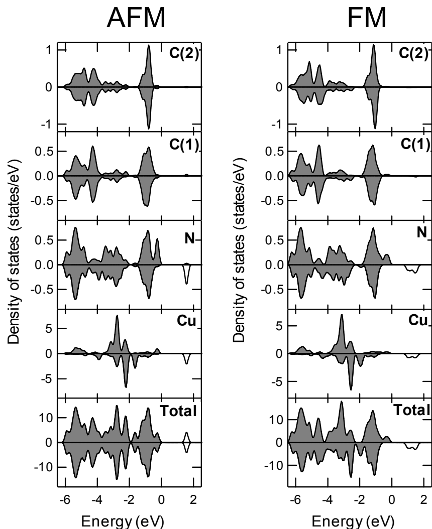
Figure 5. Spin-resolved density of states for \beta -[Cu(pz) 2 ] n . 2. Left: antiferromagnetic order; right: ferromagnetic order. Positive/negative values indicate spin up/down density of states. Filled areas indicate occupied states. Partial density of states are referred to single atoms. Atomic labels as indicated in Figure 1b.
