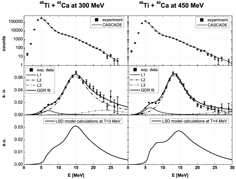
Fig. 2. Upper panel: The GDR spectra measured for ^{88}\text{Mo} at 300 MeV and 450 MeV ^{48}\text{Ti} beam energies compared to the calculations performed using Monte Carlo version of CASCADE code. Middle panel: The GDR line-shapes obtained from preliminary fits for 300 MeV and 450 MeV beam energies. The strength functions are composed of three components (also indicated in figure) showing the increase of low energy part for higher beam energy. Bottom panel: The GDR strength functions calculated using LSD model for ^{88}\text{Mo} at temperatures of T = 3 and 4 MeV for spin distributions with the average values of \langle I \rangle = 41 and 44 \hbar , respectively.
