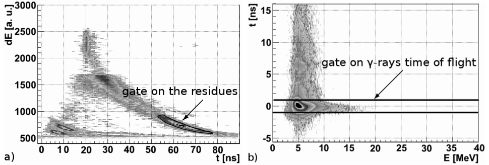
Fig. 1. (a) Energy loss ( dE ) in the first layer of the phoswich detector [16] versus time of flight. The marked region corresponds to the detection of residues. This gate is used to produce the clean high-energy \gamma -spectra. (b) The time of flight versus energy measured with the HECTOR detector. The gate indicated selects \gamma -rays without influence of neutrons energy deposits.
