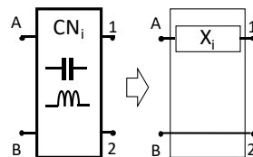
Figure 3. Example of a Series-Series (SS) compensation network.
