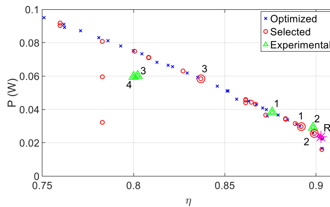
Figure 11. \eta - P_L pairs relevant to optimized (blue crosses), selected (red circles), and experimental (green triangles) C_t - C_{pu} pairs.
