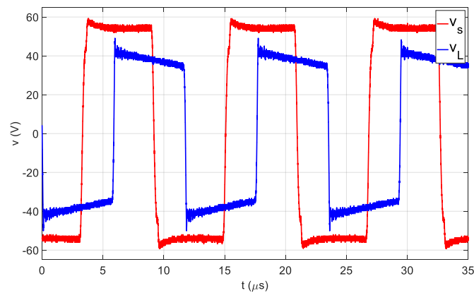
Figure 12. Voltage v_s at the output of the high frequency inverter (HFI) (red) and voltage v_L at the input of the high frequency diode rectifier (HFDR) (blue) during experiment 2.
