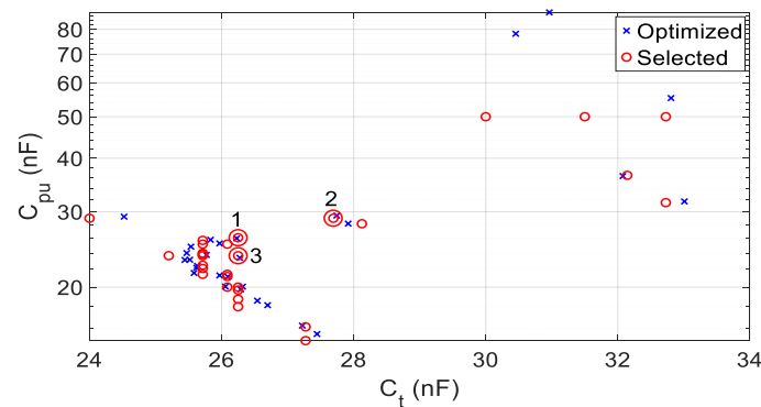
Figure 10. Optimized (blue crosses) and selected (red circles) C_t - C_{pu} pairs.
