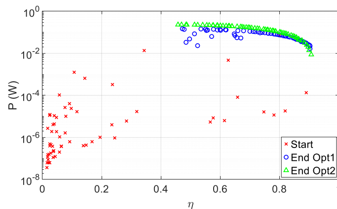
Figure 7. Improved Pareto front: individuals of the starting population (red crosses), the Pareto front of Opt1 (blue circles), and the Pareto front related to Opt2 (green triangles).
