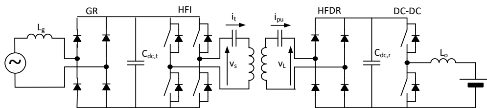
Figure 8. Schematic of the prototypal WPTS.
