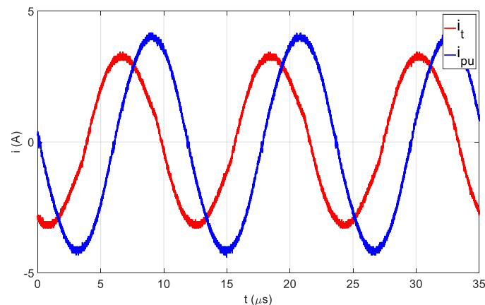
Figure 13. Current i_t in the transmitting coil and current i_{pu} in the pickup during experiment 2.
