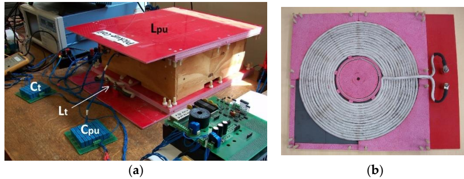
Figure 9. (a) Experimental setup. (b) Coil layout.
