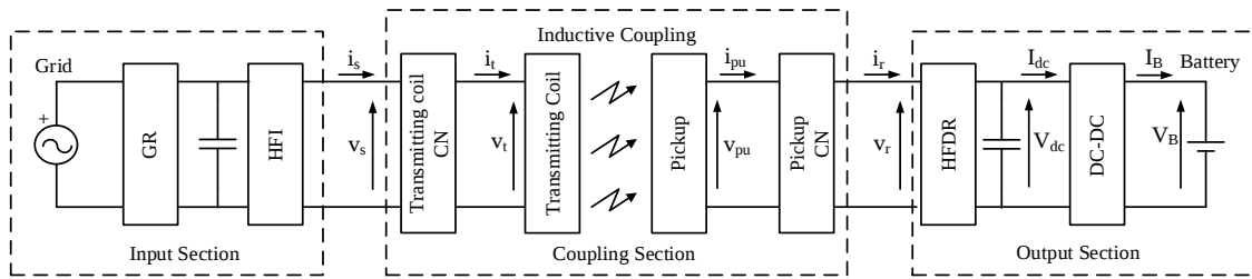
Figure 1. Circuitual scheme of a wireless power transfer systems (WPTS).
