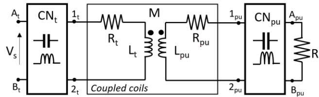
Figure 2. Circuit scheme of the coupling section of a WPTS.
