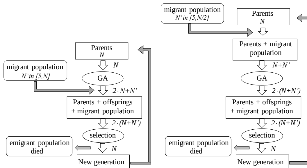
Figure 4. Optimization flow chart (left) Migration Non-Dominated-Sorting Genetic Algorithm (M-NSGA) and (right) Migration Parents-NSGA (MP-NSGA).
