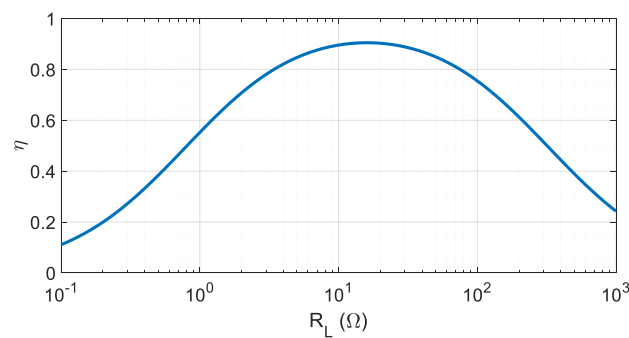
Figure 6. Power transfer efficiency vs. equivalent load resistance.
