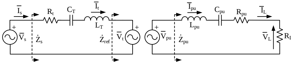
Figure 5. WPTS with SS topology.
