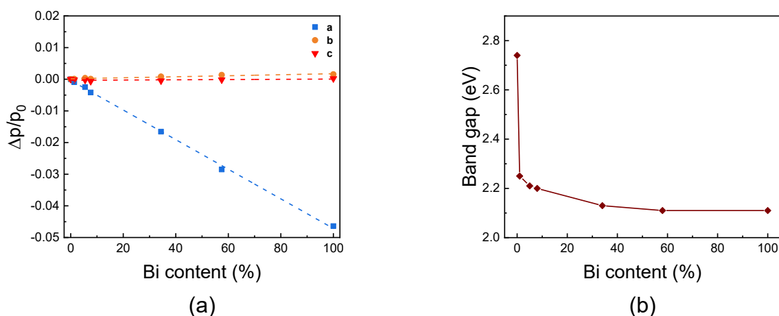
Figure 6. (a) Lattice parameter relative variation vs. %Bi [Bi content (%)], in the form of \Delta p/p_0 (where p = a, b, c and p_0 values are taken with reference to the (\text{TMSO})\text{PbI}_3 species, that with x = 0 ) for the (\text{TMSO})_3\text{Pb}_{3x}\text{Bi}_{2(1-x)}\text{I}_9 series. (b) Optical band-gap vs. %Bi.
