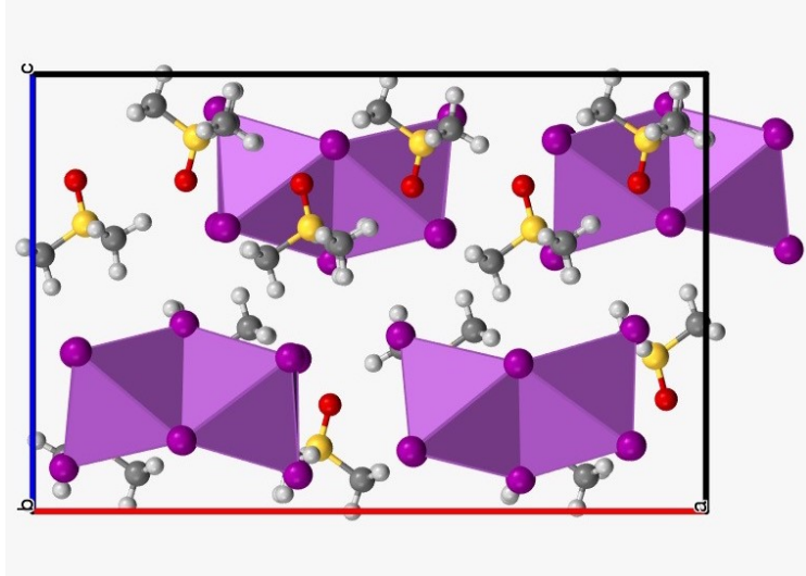
Figure 8. (\text{TMSO})_3\text{Bi}_2\text{I}_9 supercell used in the DFT calculations. Colors as in Figure 4.
