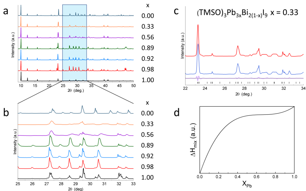
Figure 5. (a) Comparison of the raw diffraction data for the (\text{TMSO})\text{PbI}_3 , the doped (\text{TMSO})_3\text{Pb}_{3x}\text{Bi}_{2(1-x)}\text{I}_9 ( 0 < x < 1 ) and the (\text{TMSO})_3\text{Bi}_2\text{I}_9 crystal phases in the 7\text{--}50^\circ 2\theta range (bottom to top); (b) magnification of the 25\text{--}33^\circ section, where the peak-shape anomaly discussed in the text is more evident; (c) fit of the 22\text{--}34^\circ region for the (\text{TMSO})_3\text{Pb}_{0.99}\text{Bi}_{1.34}\text{I}_9 sample, where sharp peaks correspond to 0kl reflections, while “trapezoidal” regions belong to h \neq 0 ones. This phenomenological description, obtained by selective convolution of a rectangular function of unit area with a width proportional to h^2 , is physically interpreted in the Results and Discussion section. Observed data: blue dots; calculated trace: red line; difference plot and peak markers at the bottom; (d) relative enthalpy of mixing of the solid solutions as a function of the Pb molar fraction ( X_{\text{Pb}} ).
