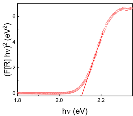
Figure 7. Tauc plots of (TMSO)PbI 3 (a), (TMSO) 3 Pb 3x Bi 2(1-x) I 9 (0 < x < 1) (b-f) and (TMSO) 3 Bi 2 I 9 (g)
