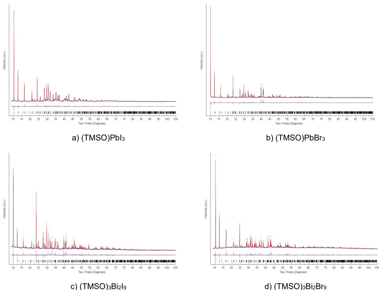
Figure 1. Rietveld refinement plots for: a) (\text{TMSO})\text{PbI}_3 , b) (\text{TMSO})\text{PbBr}_3 , c) (\text{TMSO})_3\text{Bi}_2\text{I}_9 and d) (\text{TMSO})_3\text{Bi}_2\text{Br}_9 . Observed and calculated traces in blue and red, respectively, with difference plot (in violet) and peak markers (black bars) at the bottom.
