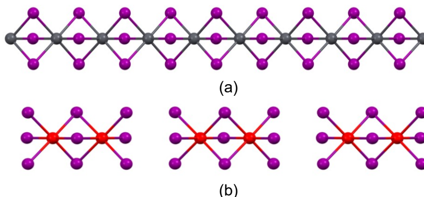
Figure 4. The atomic disposition along the a axis of: (a) 1D chains with 100% Pb 2+ ions occupancy in the infinite ([PbI 3 ] ∞ ) polyanion; (b) isolated [Bi 2 I 9 ] 3- trianions, separated by vacant B-sites. Pb in grey, Bi in red, and I in violet.
