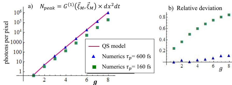
Figure 6. (a) Mean number of photons at the peak of the signal pulse \langle \hat{A}_s^{\dagger out}(\vec{\xi}_M) \hat{A}_s^{out}(\vec{\xi}_M) \rangle \times dx^2 dt (units are photons per numerical pixel). The red line is the QS model prediction in Eq. (17), where the integral was calculated via a discrete sum over the same numerical grid of the simulations. The symbols are the results of simulations. (b) Relative deviation between analytic predictions and numerical results
