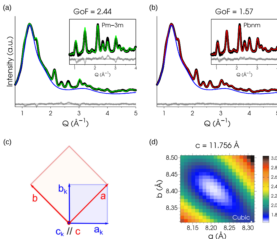
Figure 2. WAXTS-DSE (room-temperature) crystal structure analysis of ultrasmall colloidal 5 nm CsPbBr 3 NCs. Best fit using a) the cubic Pm-3m and b) the orthorhombic Pbnm crystal structure models: experimental data (black dots), DSE pattern model (green and red traces), toluene (blue trace), residual (grey trace). c) Geometrical relationship between the orthorhombic ( a , b , c ) and cubic ( a k , b k , c k ) unit cell vectors of LHP in the ab -plane; The c and c k axes, drawn out of the page, are parallel. d) 2D map of GoF (in colour-grade) vs orthorhombic a and b lattice parameters (at c = 11.756 Å). The minimum GoF is found at a = 8.207(1) Å and b = 8.407(1) Å ( a/b = 0.976). The refined cell parameter of the Pm-3m model ( a k = 5.875 Å = \frac{8.308}{\sqrt{2}} Å) is highlighted by the white spot in the map (bottom-right corner). For the estimation of uncertainties, details are given in the Supporting Information.
