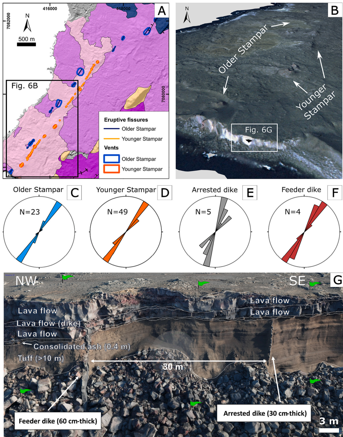
Fig. 6. A) Detailed map of the Older and Younger Stampar crater rows, with the strike of the eruptive fissures inferred by the elongation of each vent. For lava units, see the legend in Fig. 2A. Spatial reference: WGS 84 – UTM zone 27 N. B) View of the 3D model obtained from historical aerial photographs (location in Fig. 6A), where the absence of tension fractures and faults can be noticed. Rose diagrams showing the strike of C) the Older Stampar eruptive fissures, D) the Younger Stampar eruptive fissures, and of the outcropping segments of E) the arrested and F) the feeder dike. G) UAV-derived 3D model of the outcrop, with the layers and the two dikes highlighted (location in Fig. 6B). Ground Control Points (GCPs) used to georeference the model are shown as green flags. (For interpretation of the references to colour in this figure legend, the reader is referred to the web version of this article.)
