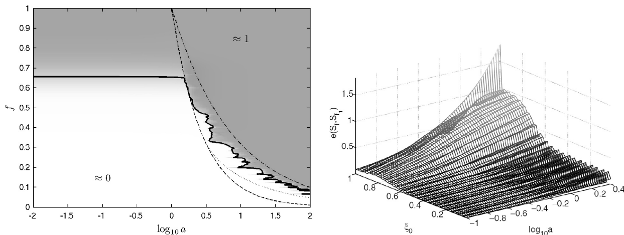
Fig. 3. EMD, left, and Synchrosqueezing, right, performance measure of separation for two-tones original images shown in [17] and [18].
