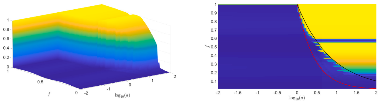
Fig. 6. Left panel, IF performance in separating two-tones with irrational frequencies from signal (14), when the currently implemented approach for mask length selection is used. The results shown are obtained using criterion (23) when \phi = 3 . Right panel, the projection onto the (a, f) -plane. The critical curves af = 1 and af^2 = 1 are plotted in solid red and black, respectively. From these plots we see that the performance of IF fits well with what predicted by formulas presented by Flandrin et al. in [17].
