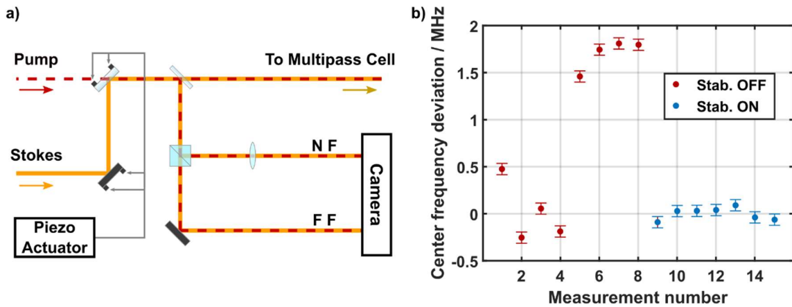
FIGURE 6. Active beam alignment. a) Schematic diagram of the active beam alignment system; NF: near field; FF: far field. b) Fluctuations of the line center frequency over different measurements with the gas kept at constant thermodynamic conditions and the Stokes beam misaligned and realigned onto the pump beam before each measurement. Red dots (measurements 1-8) represent measurements where the alignment is manual, while blue dots (9-15) represent measurements under active beam alignment. Each dot corresponds to an averaged spectrum acquired over 5 min, while error bars are the standard deviation of the mean. The vertical scale is relative to the mean line center frequency retrieved with active stabilization.
