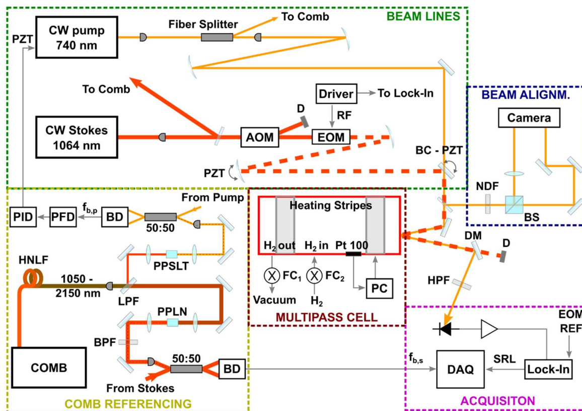
FIGURE 1. Optical layout of SRS the spectrometer. Colored boxes enclose the parts of the setup described in detail in the sections of the main text. AOM: acousto-optic modulator; D: (beam) dump; EOM: electro-optical modulator; RF: radiofrequency signal; PZT: piezoelectric actuator; BC: beam combiner; DM: dichroic mirror; HPF: high-pass filter; BS: beam splitter; NDf: neutral density filter; SRL: stimulated Raman loss signal; DAQ: digital acquisition board; BD: balanced detector; LPF: low-pass filter; BPF: band-pass filter; PPLN: periodically-poled lithium niobate crystal; PPSLT: periodically-poled stoichiometric lithium tantalate crystal; PFD: phase-frequency detector; PID: proportional-integral-derivative controller.
