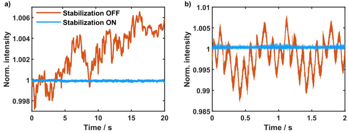
FIGURE 4. Active stabilization of laser power. Power fluctuations of the Stokes beam relative to the power at t = 0 s when the active stabilization is inactive (red trace) or active (blue trace), in the case of fixed Stokes laser frequency (a) and scanning Stokes frequency (b) over about 10 GHz at a rate of 1 Hz.
