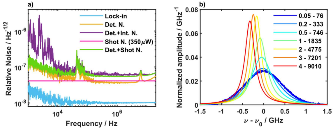
FIGURE 3. Noise performance. a) Comparison of the detection noise with the shot noise level. From top to bottom in the legend: lock-in noise floor, detector noise (Det. N), detector + laser intensity noise(Int. N), shot noise calculated for the pump power impinging on the detector (350 \mu W), detector + shot noise added in quadrature. b) Normalized SRL spectra of the Q(1) 1-0 line of H_2 measured at different pressures. The first number in the legend represents the measurement pressure in bar, the second one is the SNR of the spectrum.
