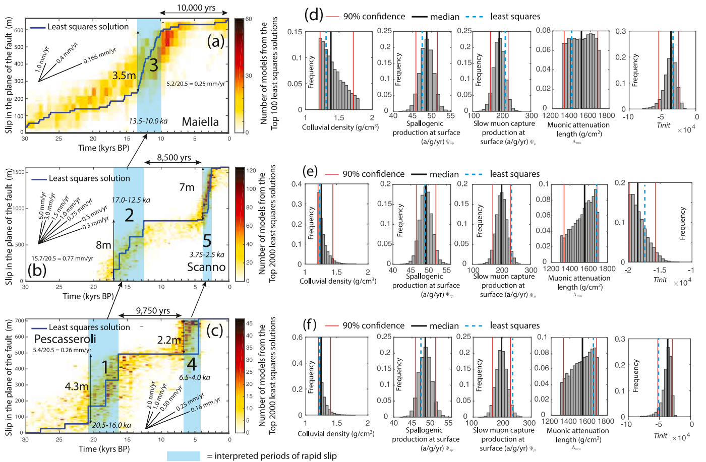
Fig. 5. Details of how the slip-histories were recovered and interpreted. (a), (b) and (c) Slip in the plane of the fault indicated by the least squares solutions derived from MCMC modelling of the 36 Cl data. (d), (e) and (f) Medians and 90% confidence from the posterior distributions for colluvial density, spallogenic production, slow muon capture and age from which production is preserved ( T_{init} ), and the values for the least squares solution. In (a), (b) and (c) blue rectangles show an interpretation of periods of rapid slip. Numbers and arrows show our interpretation of how periods of rapid slip migrated between the 3 faults through time. The exact values for the time duration of the periods of rapid slip and the value of slip are subjective (see also Fig. 4), and this is discussed in the text. (For interpretation of the references to colour in this figure legend, the reader is referred to the Web version of this article.)
