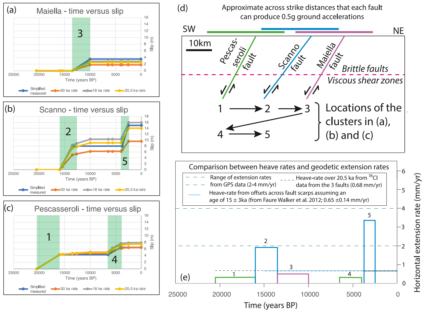
Fig. 9. Summary of the migration of periods of rapid slip across the strike of the Apennines, and comparison with strain-rates implied by GPS data, the summed rate averaged over \sim 20 ka constrained by ^{36}\text{Cl} data, and the summed rate assuming the total offset across the scarps accumulated in 15 \pm 3 ka. (a), (b) and (c) Five periods of rapid slip have been measured and replicated via modelling. (d) Locations of the periods of rapid slip through time and the approximate width across strike that is implied to experience \sim 0.5 g horizontal accelerations, assuming this extends 20 km into the hangingwall and 10 km into the footwall of a fault that ruptures in an earthquake. Fault dips are from field measurements of the surface outcrop of the fault plane. (e) Slip-rates within each period of rapid slip-rate converted into heave rates using the measured fault dip. Assuming a 4 mm/yr regional extension rate the faults have individually taken up between 8% and 84% of the regional extension. Assuming a 2 mm/yr regional extension rate the faults have individually taken up between 15% and 169% of the regional extension rate. Assuming a 0.68 mm/yr extension rate, constrained by ^{36}\text{Cl} , the faults have individually taken up between 44% and 496% of the regional extension rate.
