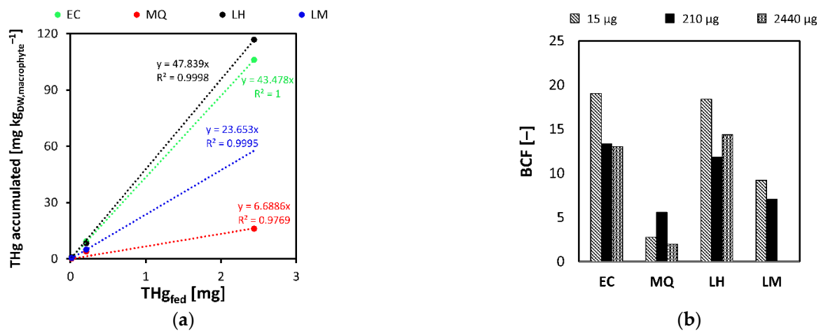
Figure 4. (a) THg accumulated in macrophytes as a function of THg fed and (b) BCF after 27 d as a function of the type of macrophyte and THg fed .
