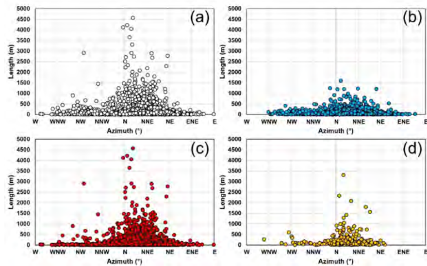
Figure 8. Graphs showing the relation between the strike and length of (a) all structures, (b) extension fractures, (c) normal faults and (d) eruptive fissures.
