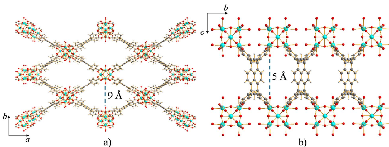
Fig. 2 Representation of the crystal structure of NU-901: (a) portion of the framework viewed approximately along the crystallographic c -axis; highlighted the width 62 of the rhombic microporous channels. (b) Portion of the framework viewed along the crystallographic a -axis; highlighted the width of the rhombic windows. Element colour code: C, dark grey; H, light grey; O, red; Zr, cyan. Crystallographic information retrieved from 53.
