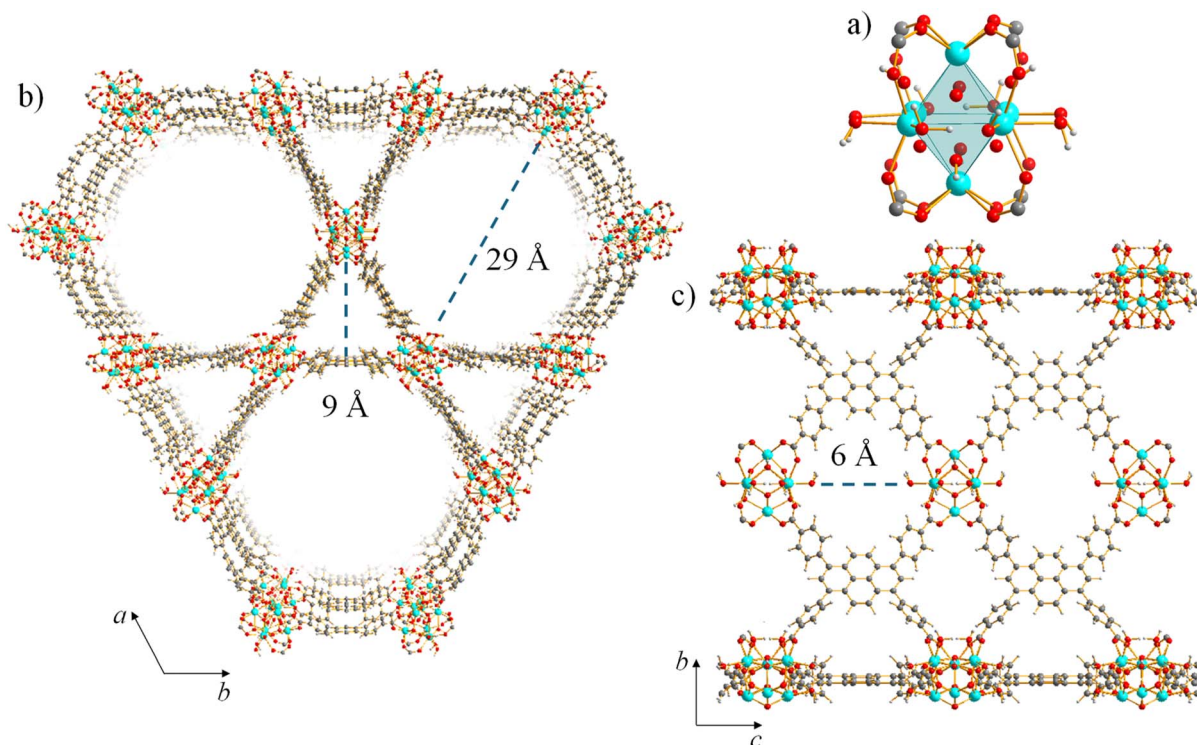
Fig. 1 Representation of the crystal structure of NU-1000: (a) the node. (b) Portion of the framework viewed approximately along the crystallographic c -axis; highlighted the width 60 of the microporous and mesoporous channels. (c) Portion of the framework viewed along the crystallographic a -axis; highlighted the width 61 of the rhombic window. Element colour code: C, dark grey; H, light grey; O, red; Zr, cyan. Crystallographic information retrieved from 37.
