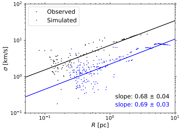
Figure 2. Size–linewidth relation in the synthetic HNC O( 4_{04}\text{--}3_{03} ) emission map of the simulation snapshot (data from Petkova et al. 2023, blue) and the Brick cloud (data from Rathborne et al. 2015, black). The individual data points correspond to structures identified within the corresponding PPV cubes using dendrograms. Power-law fits for the two data sets are shown as solid lines, with both slopes being \approx 0.7 .
