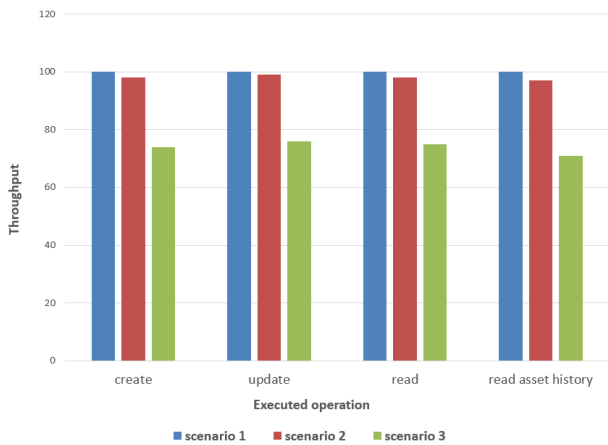
Figure 15: Network throughput - test-bed
