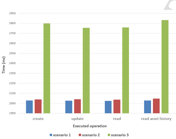
Figure 11: Time required to execute the operations on the ledger - test-bed
