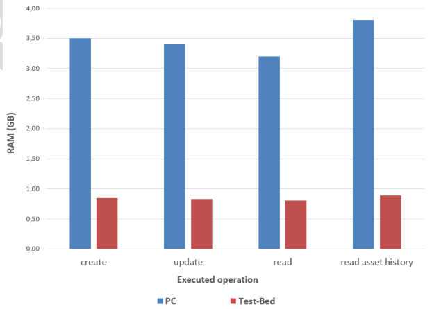
Figure 13: Average RAM occupancy - scenario 3
