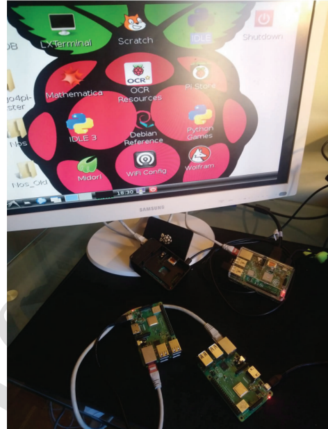
Figure 9: Test-Bed representation
