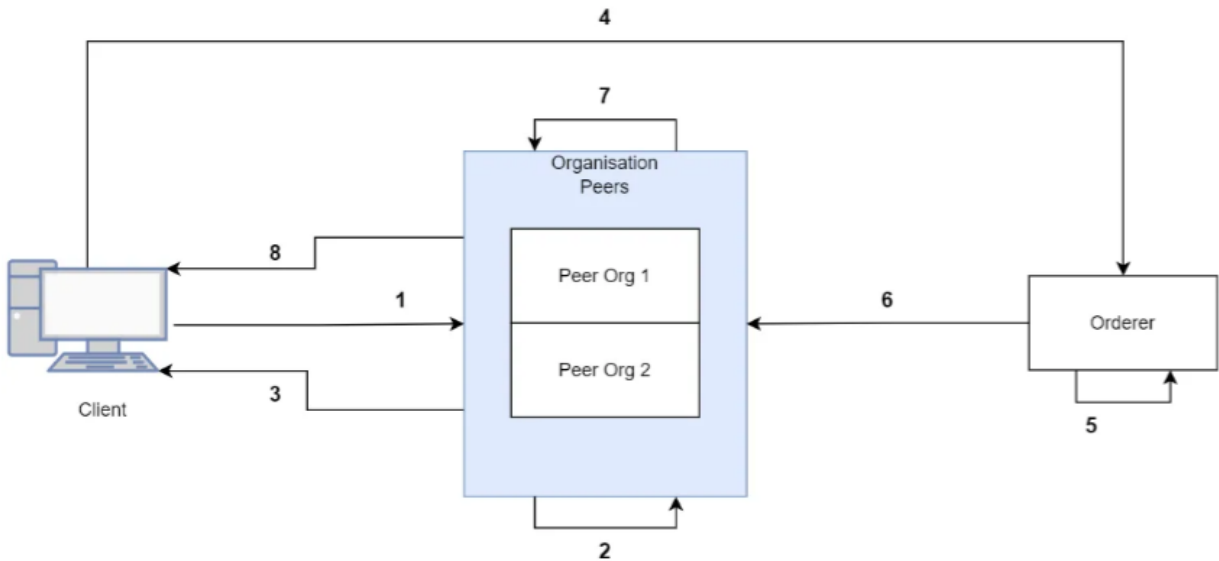
Figure 4: Consensus schema
