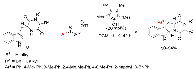
Scheme 15. Diastereoselective arylation of tryptophan derivatives.
