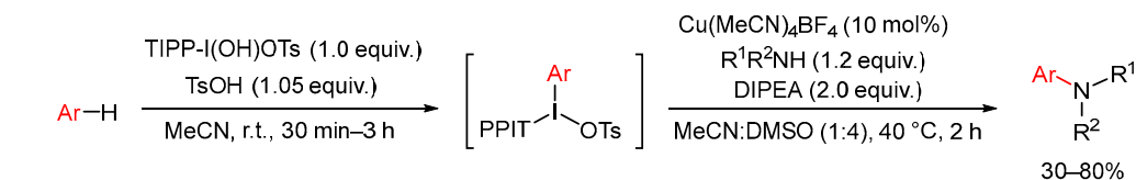
Scheme 85. Copper(I)-catalyzed C-H amination of unsymmetric diaryliodonium salts with amine compounds.
