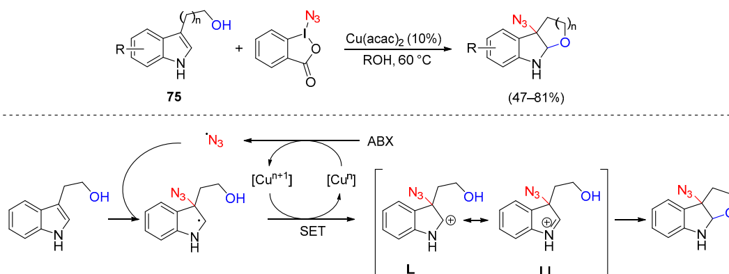
Scheme 101. Intramolecular copper-catalyzed alkoxyazidation of tryptophols.
