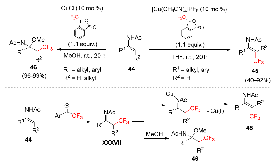
Scheme 47. Trifluoromethylation of electron-rich enamides.
