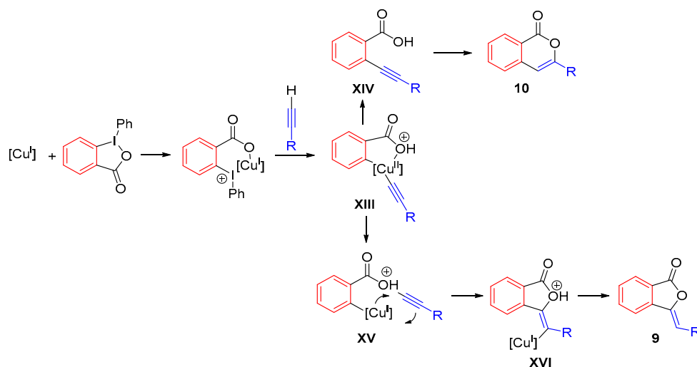
Scheme 18. Proposed mechanism for the conversion of terminal alkynes into phthalides and isocoumarins.
