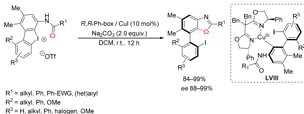
Scheme 111. Copper-catalyzed benzoxazoles formation with cyclic diaryliodonium compounds.
