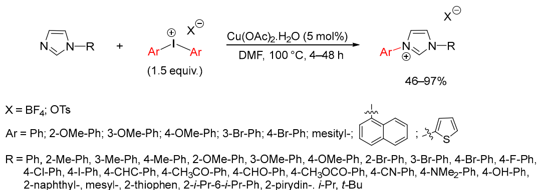
Scheme 87. Aryl quaternization of imidazole derivatives under copper catalysis.
