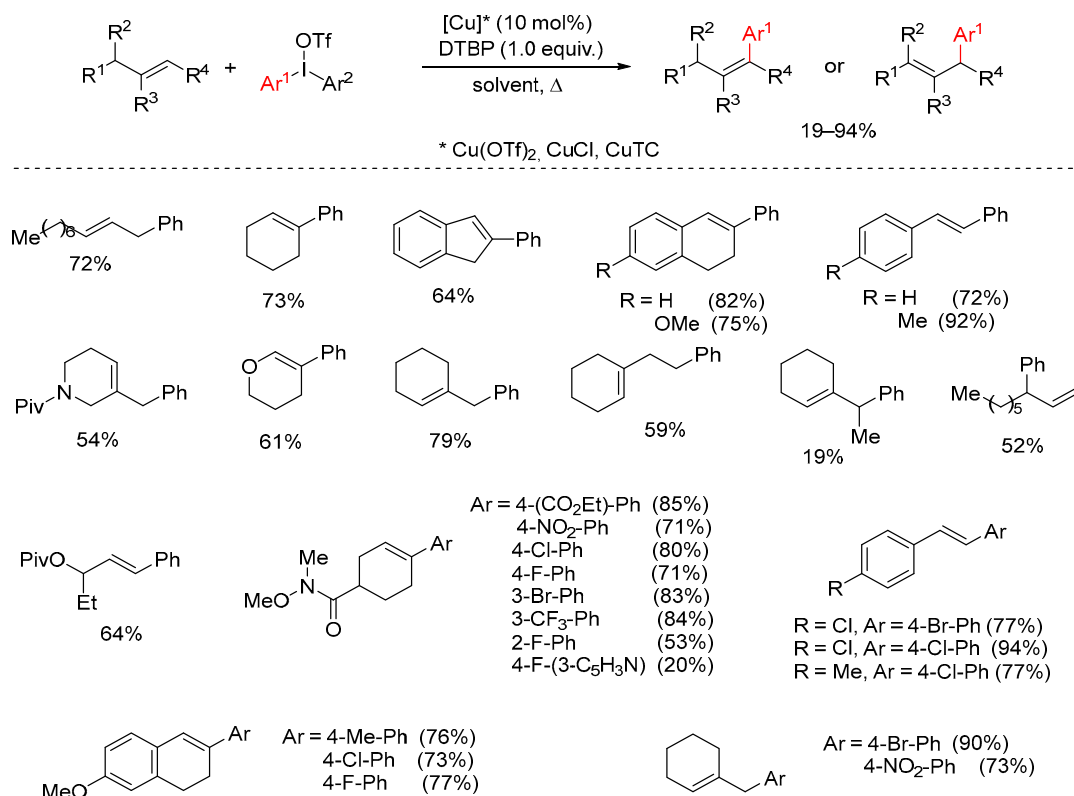
Scheme 16. Copper-catalyzed arylation of alkenes with diaryliodonium salts.
