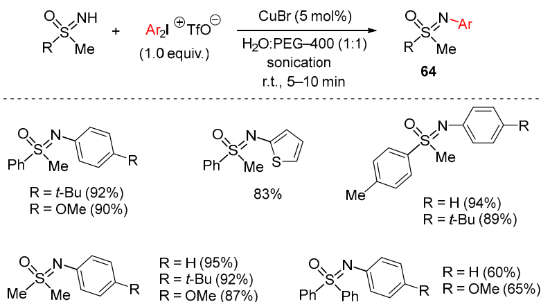
Scheme 83. Copper(I)-catalyzed arylation of sulfoximines with diaryliodonium salts.
