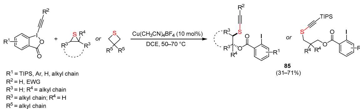
Scheme 116. Copper-catalyzed synthesis of aryltrifluoromethylsulfones.
