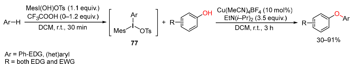
Scheme 104. Copper(I)-catalyzed C-H oxyarylation of phenol derivatives.
