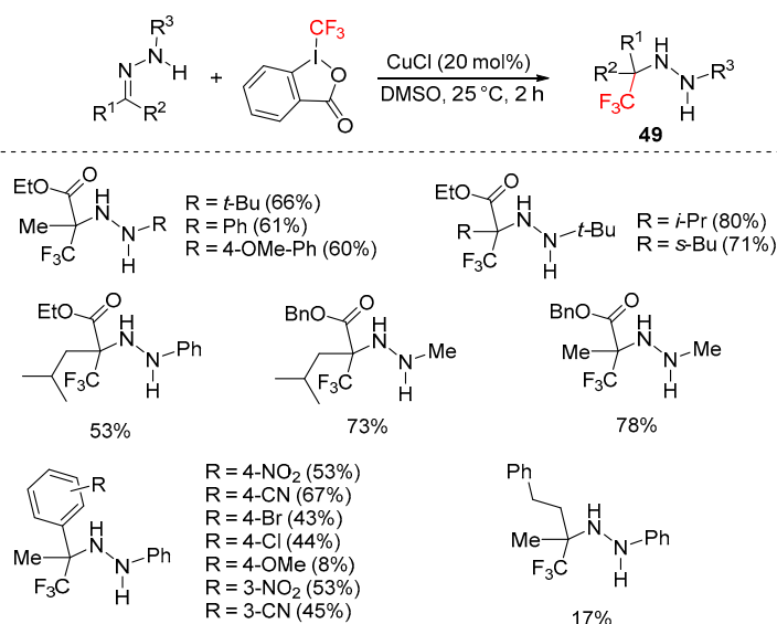
Scheme 54. Trifluoromethylation of N -monosubstituted hydrazones.
