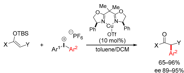
Scheme 13. Enantioselective \alpha -arylation of N -acyloxazolidinones.
