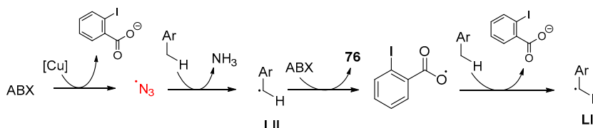
Scheme 102. Azidation of styrene-type double bond ( path a ) and benzylic C-H bonds ( path b ) with ABX under copper-photoredox catalysis.
