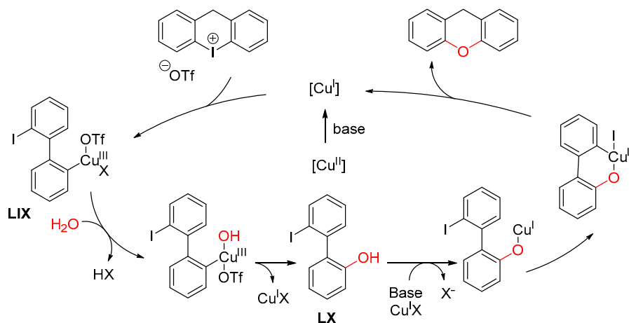
Scheme 112. Copper-catalyzed water insertion into cyclic diaryl iodonium reagents.
