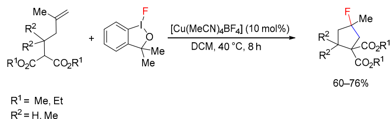
Scheme 122. Hypervalent iodine as reagent in fluorocyclization.
