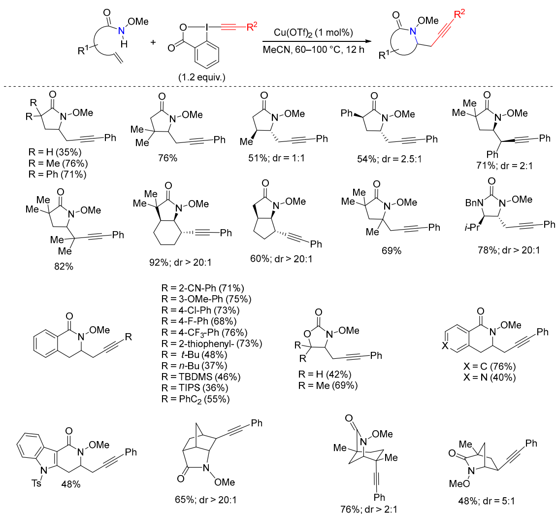
Scheme 37. Cu-catalyzed aminoalkynylation of alkenes with EBX.
