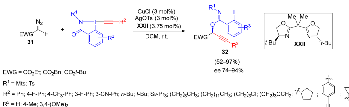
Scheme 34. Copper-catalyzed enantioselective oxyalkynylation of diazo compounds.
