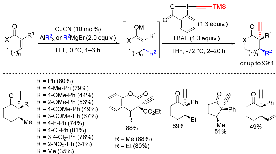
Scheme 38. Sequential Michael addition/electrophilic alkynylation on \alpha,\beta -unsaturated cyclic ketones.
