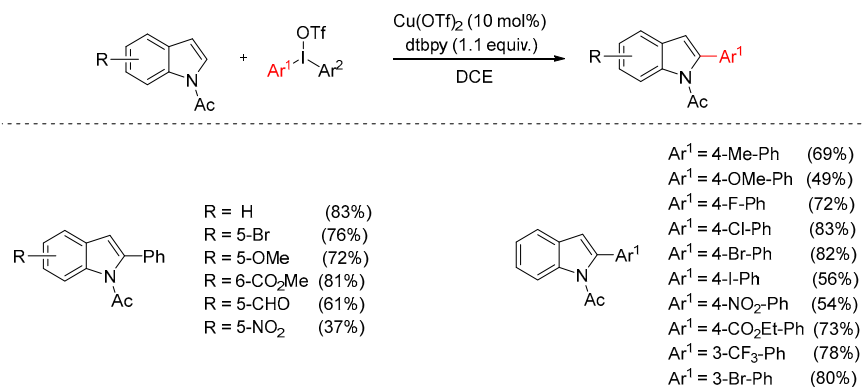
Scheme 5. Selective Cu(OTf) 2 -catalyzed C2-arylation of N -acetylindoles.
