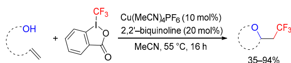
Scheme 69. Oxytrifluoromethylation of unactivated alkenes.
