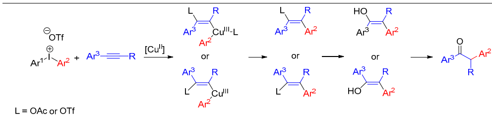
Scheme 19. Arylation reaction of internal alkynes with diaryliodonium salts to \alpha -arylktones.
