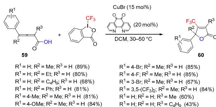
Scheme 72. Copper-catalyzed oxytrifluoromethylation of 2,3-allenoic acids.
