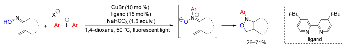
Scheme 97. Copper-catalyzed synthesis of N -aryl-isoxazolidines.
