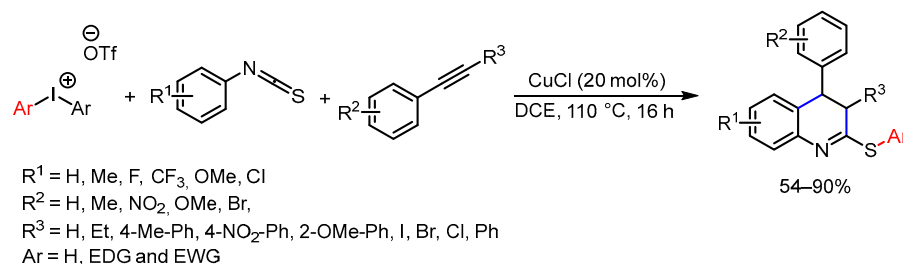
Scheme 121. Synthesis of quinoline derivatives.
