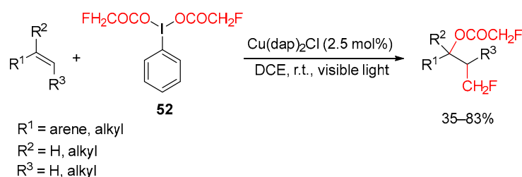
Scheme 64. Copper-catalyzed oxy-monofluoromethylation of alkenes.
