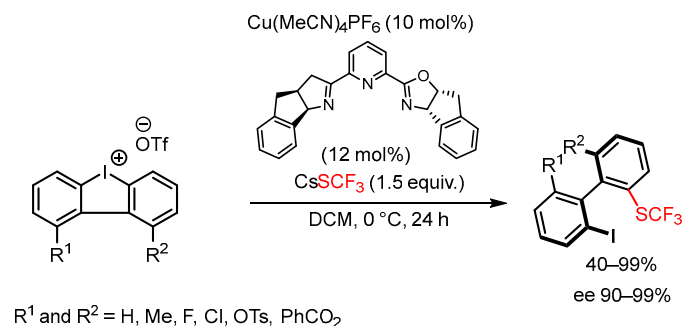
Scheme 120. Atroposelective synthesis of trifluoromethylthiolated biaryls.
