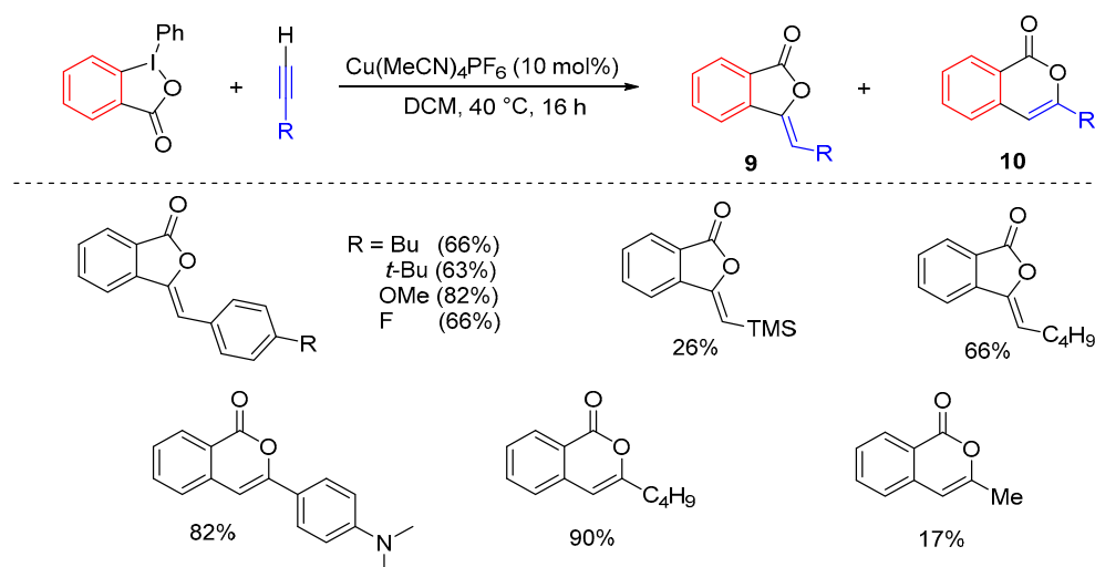
Scheme 17. Access to phthalides and isocoumarins from terminal alkynes.
