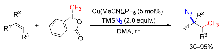
Scheme 65. Copper mediated trifluoromethylazidation of alkenes.
