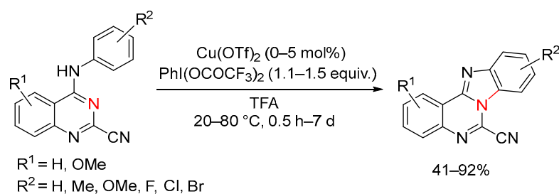
Scheme 128. Copper(II)-mediated oxidative ring closure of 4-anilinoquinazoline-2-carbonitriles.
