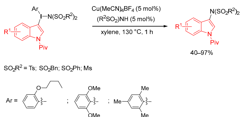
Scheme 84. Copper(I)-catalyzed C-N coupling reaction using indolyl(aryl)iodonium imides.
