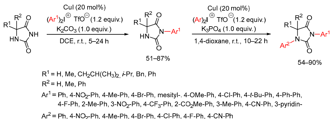
Scheme 81. Copper(I)-catalyzed arylation of hydantoins.
