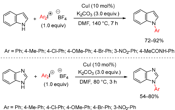
Scheme 78. Copper(I)-catalyzed arylation of indole and benzimidazole.
