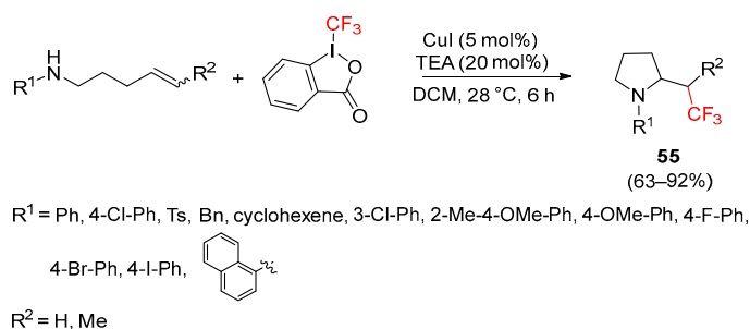
Scheme 67. Synthesis of \beta -trifluoromethylamines.
