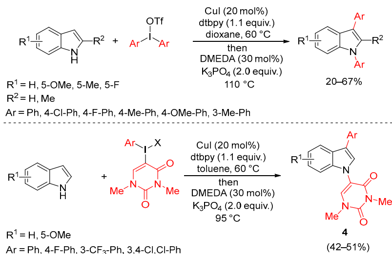
Scheme 9. Tandem diarylation of indoles.
