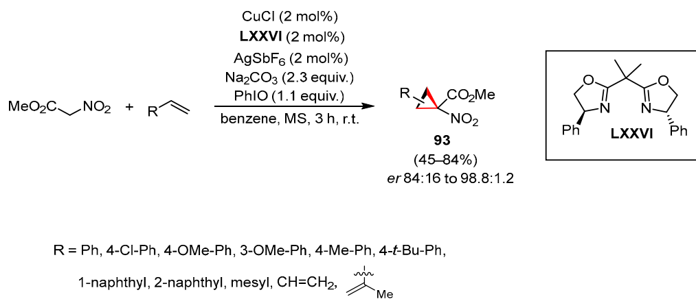
Scheme 131. Copper-catalyzed cyclopropanation reaction.
