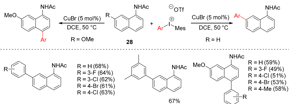
Scheme 30. C4 and C7 arylation of naphthyl-1-acetamides.
