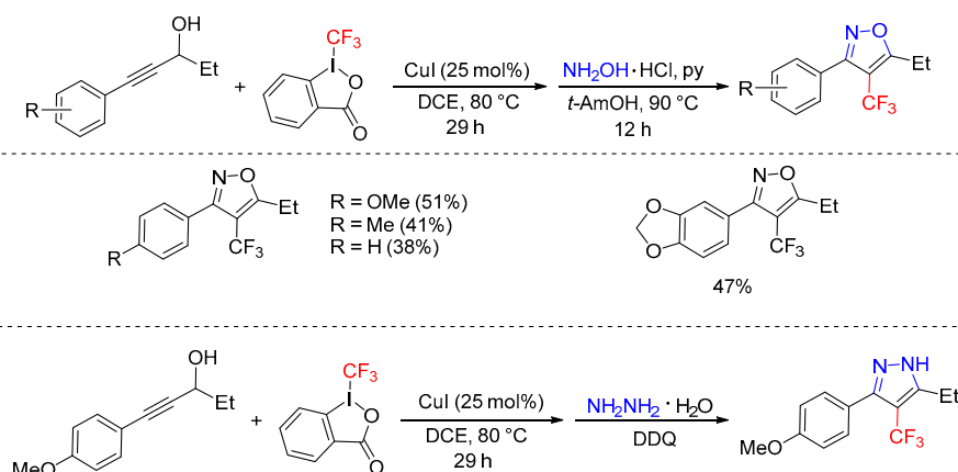
Scheme 58. Copper-catalyzed domino trifluoromethylation/Meyer–Schuster rearrangement.
