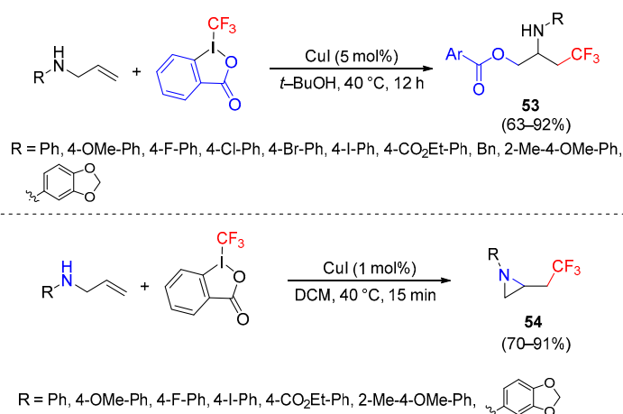
Scheme 66. Synthesis of \beta -trifluoromethylamines.
