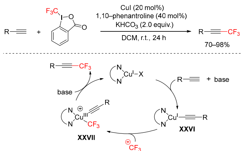
Scheme 46. Trifluoromethylation of terminal alkynes.
