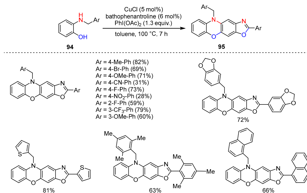
Scheme 134. Dimerization/cyclization of 2-benzylaminophenols.
