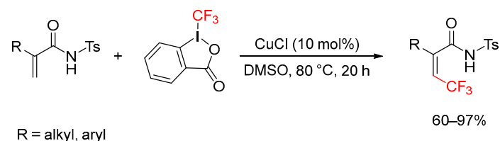
Scheme 48. Trifluoromethylation of electron-deficient alkenes.
