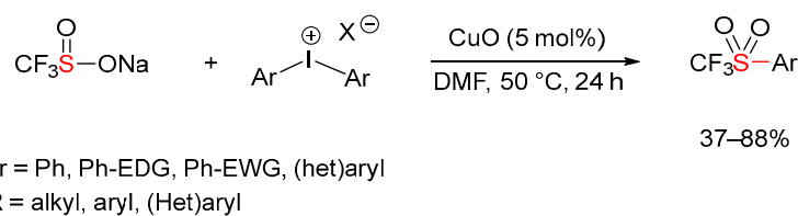
Scheme 116. Copper-catalyzed synthesis of aryltrifluoromethylsulfones.
