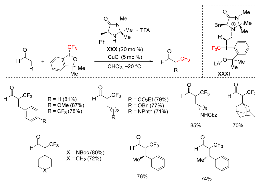
Scheme 52. Enantioselective \alpha -trifluoromethylation with organocatalyst.
