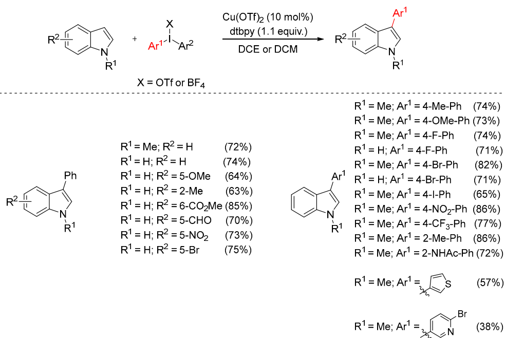
Scheme 4. Cu(OTf) 2 -catalyzed C3-arylation of indoles.
