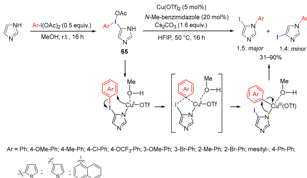
Scheme 86. Copper catalyzed aryl migration: selective synthesis of N -aryl-5-iodoimidazoles.
