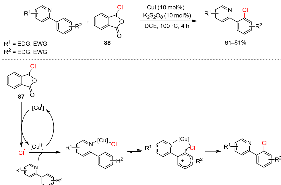
Scheme 123. Regioselective chlorination of C-H aromatic bonds.
