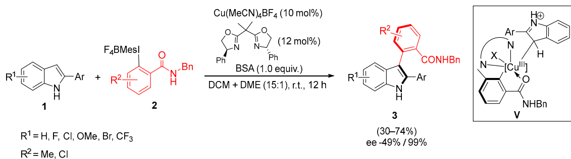
Scheme 7. Atroposelective synthesis of 2,3-diarylidoles.
