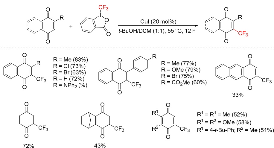
Scheme 50. Trifluoromethylation of quinones.
