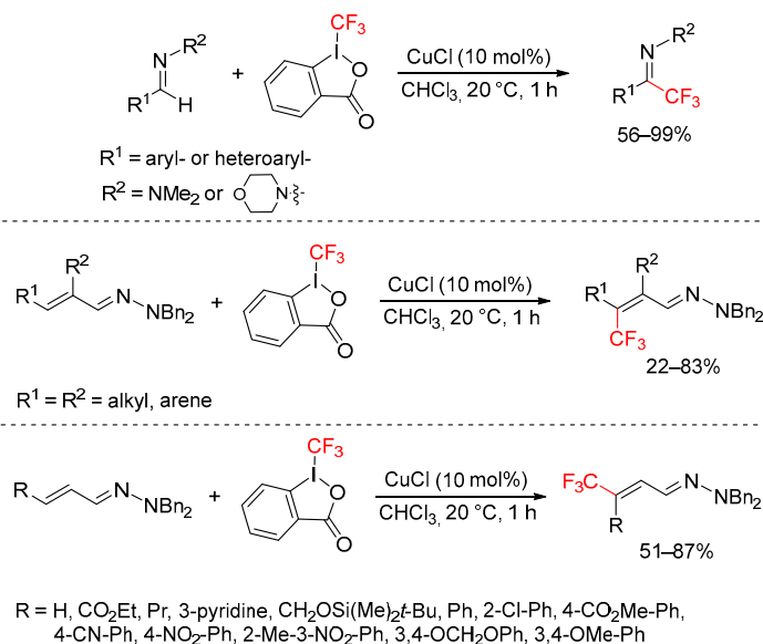
Scheme 53. Copper-catalyzed trifluoromethylation of hydrazones.
