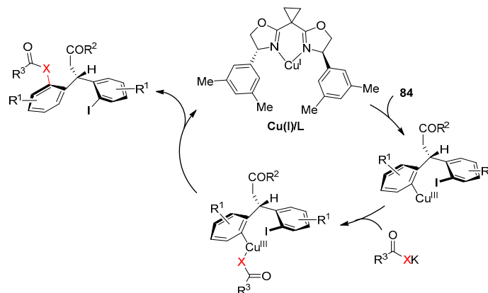
Scheme 115. Cu-catalyzed enantioselective diarylmethanes formation.
