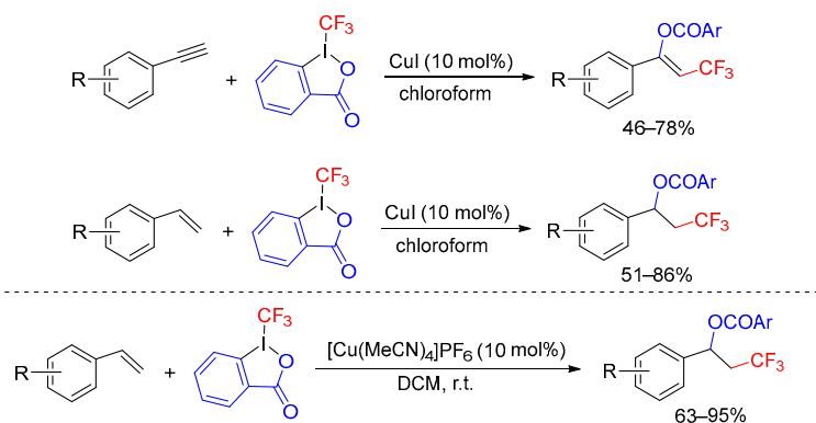
Scheme 63. Oxytrifluoromethylation of alkenes and alkynes.
