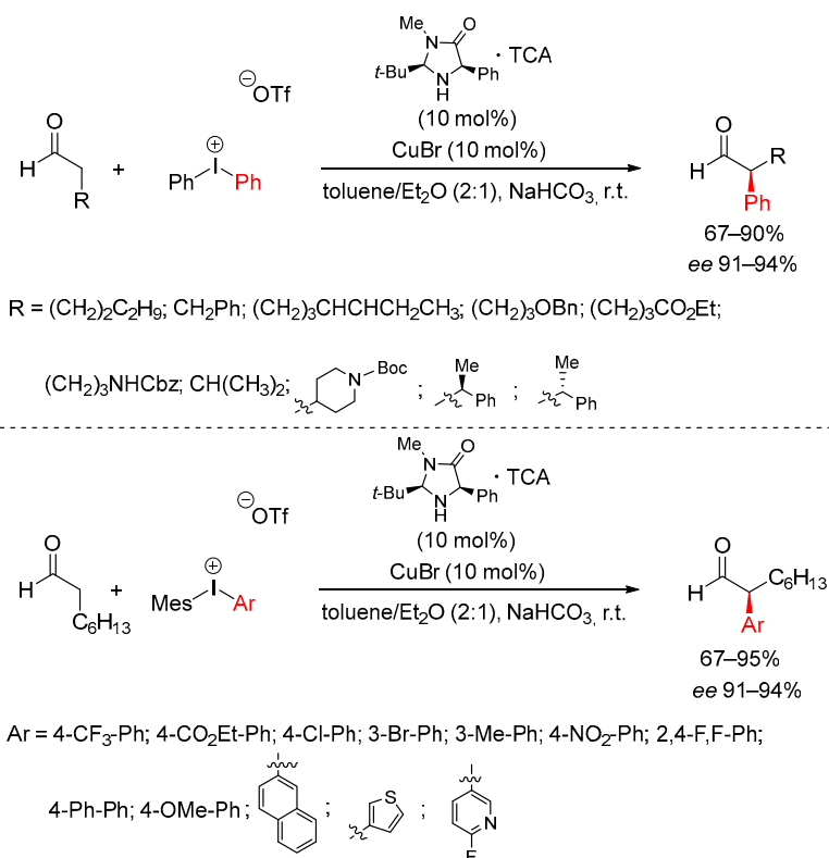
Scheme 10. Stereoselective arylation of enolizable aldehydes.
