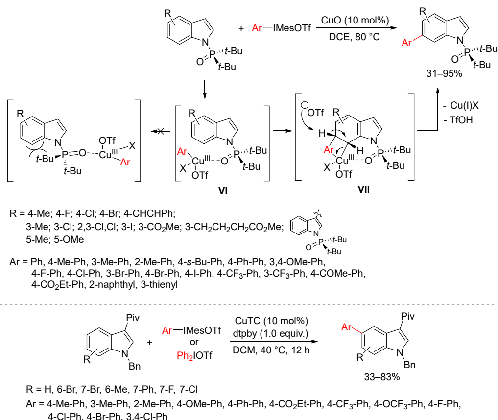
Scheme 8. Selective C5- and C6-arylation of substituted indoles.
