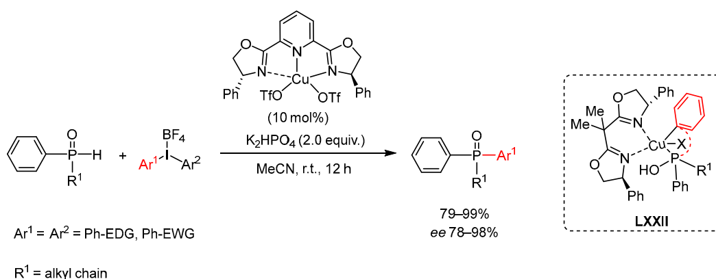
Scheme 126. Enantioselective copper-catalyzed P-Arylation using diaryliodonium reagents.
