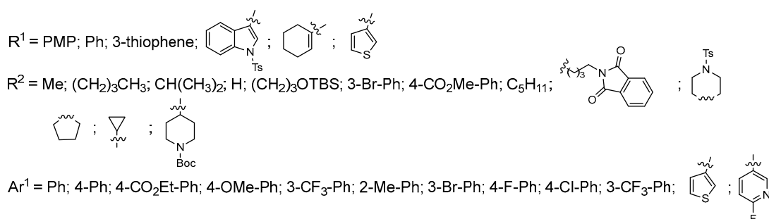
Scheme 25. Copper-catalyzed Meyer–Schuster rearrangement of propargyl alcohols.
