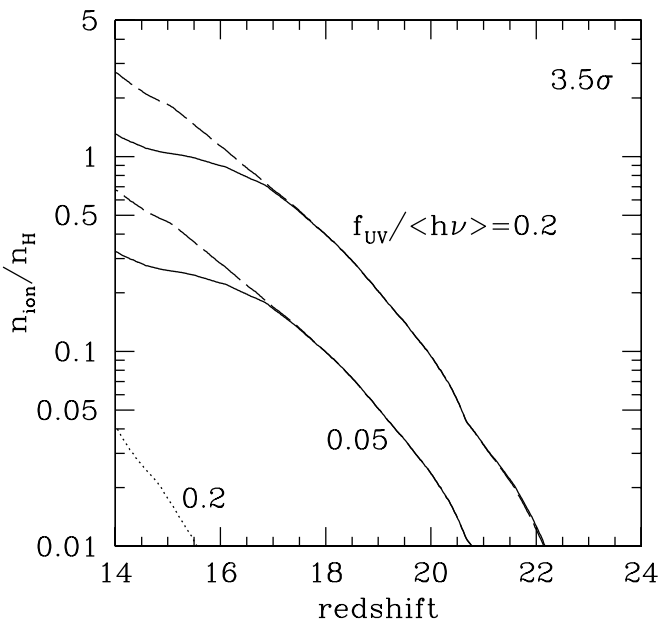
FIG. 4.—Cumulative number of ionizing photons per hydrogen atom produced by miniquasars, for different values of the fraction f_{\text{UV}} of the bolometric power that is emitted as radiation above 1 ryd with mean energy \langle h\nu \rangle (in ryd). Solid curves : In each major merger the BH in the main halo accretes a mass \Delta m_{\text{acc}} = 2m_{\text{BH}} . Dashed curves : Same with \Delta m_{\text{acc}} = 10^{-3}M_h . Dotted curve : Same with \Delta m_{\text{acc}} = 10^{-3}M_h , f_{\text{UV}}/\langle h\nu \rangle = 0.2 \text{ ryd}^{-1} , but with gas accretion suppressed in minihalos with virial temperature T_{\text{vir}} \lesssim 10^4 \text{ K} .
