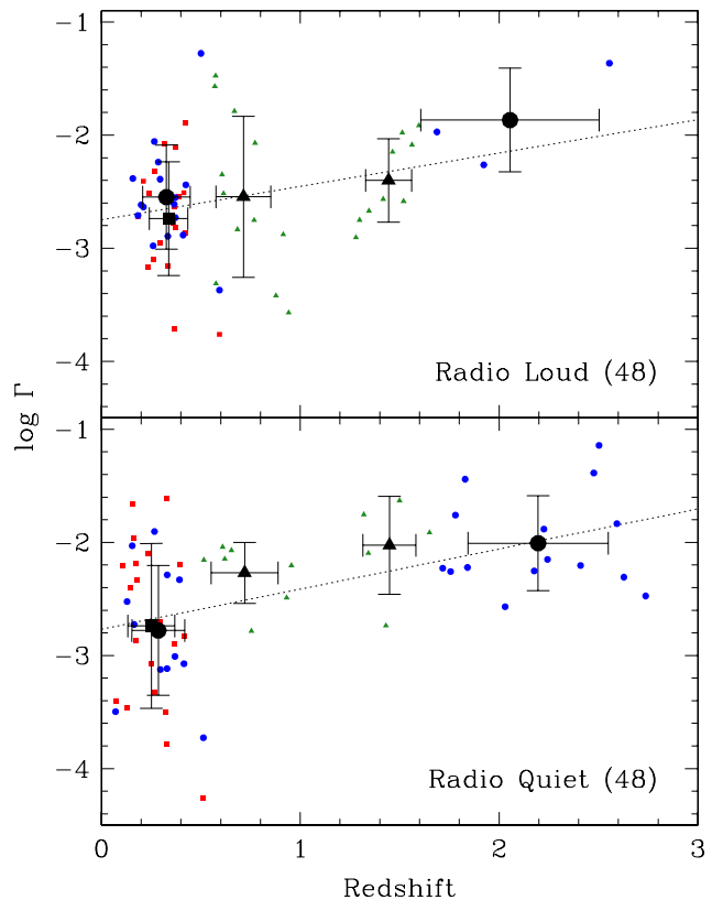
Figure 3. The redshift dependence of \Gamma for Radio Loud ( top panel ) and Radio Quiet quasars ( bottom panel ) separately. The symbol code is the same as in Figure 2. The number of objects in each subsample is also provided in parenthesis.
