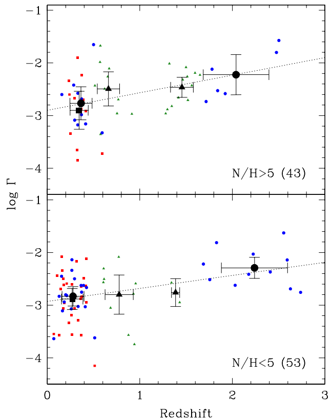
Figure 7. The same as Figure 3, for objects with N/H > 5 (top panel) and N/H < 5 (bottom panel). Again, no significant difference is reported.
