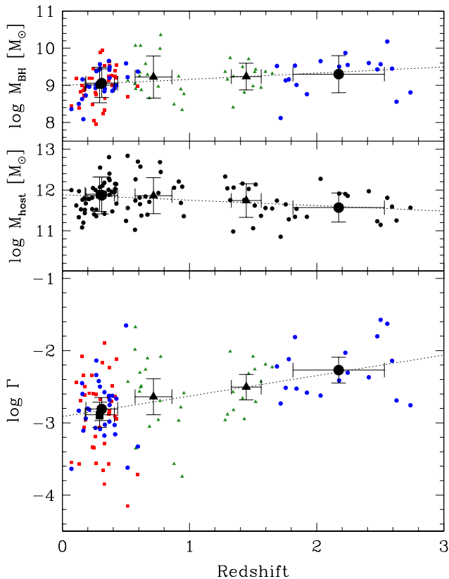
Figure 2. The redshift dependence of \mathcal{M}_{\text{BH}} ( top panel ), \mathcal{M}_{\text{host}} ( middle panel ) and their ratio \Gamma ( bottom panel ). The symbol code follows Figure 1. The best linear fits are plotted. The average points with rms as error bars of the H \beta subsample (big square), of the low- and high- z C IV data (big circles) and of the Mg II data with redshift < 1 and > 1 (big triangles) are also shown.
