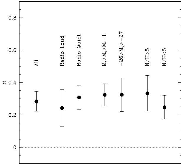
Figure 4. The slope of the \log \Gamma versus z linear fit in our data, for each subsample. Error bars are the 1\text{-}\sigma uncertainties as derived from the fit algorithm (see Table 2). All the subsets have consistent slopes around \sim 0.3 dex. A non-evolving scenario (horizontal, dotted line) mismatches with the observations in all the cases.
