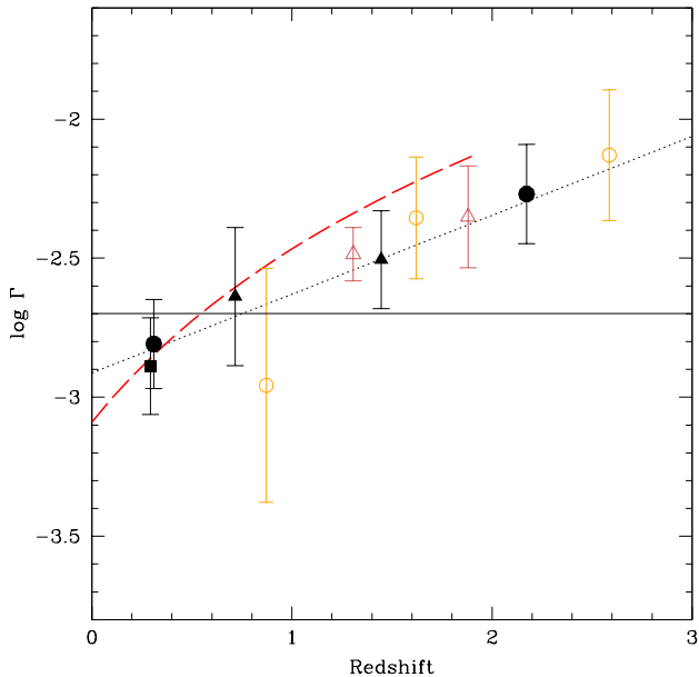
Figure 8. The average values of \Gamma for the quasars in our sample (filled symbols), together with the linear best fit (dotted line). Error bars are the 2\text{-}\sigma uncertainties in the average values for each data bin. For a comparison, the trend found in the study of radio loud AGN by McLure et al. (2006) is plotted as a dashed line. We also plot the average \Gamma values of the 51 lensed and non-lensed quasars from Peng et al. (2006a,b, empty circles) and of the 89 AGN from Merloni et al. (2009, empty triangles). The horizontal solid line represents the constant \Gamma = 0.002 case. All together the data depict a clear increase of \Gamma with z .
