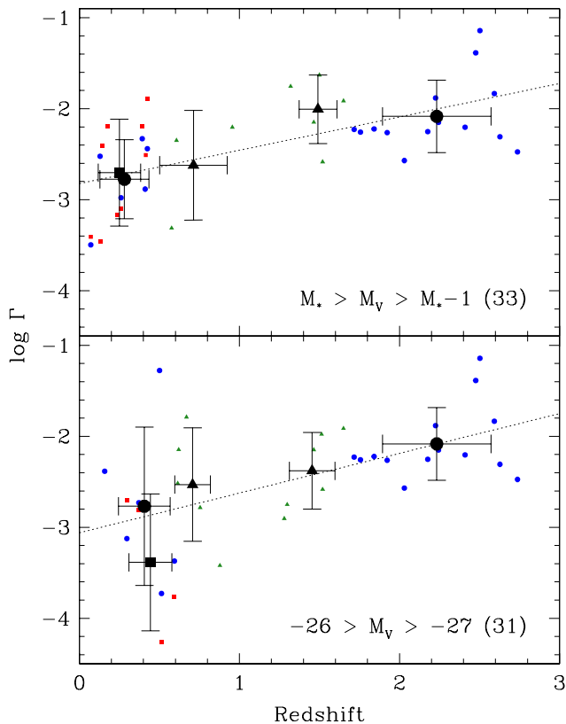
Figure 6. The same as Figure 3, for objects with M_* > M_V > M_* - 1 (top panel) and with -26 > M_V > -27 (bottom panel). No significant difference is observed in the two subsets.
