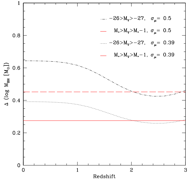
Figure 5. The bias on the prediction of \mathcal{M}_{\text{BH}} from the \mathcal{M}_{\text{BH}}-L_{\text{host}} relation with respect to the expectation from the luminosity functions of galaxies and quasars, plotted as a function of redshift. The bias estimates are obtained by integrating the luminosity function of quasars over the adopted luminosity cuts: -26 > M_V > -27 (dot-dashed and dotted lines) and M_* > M_V > M_* - 1 (dashed and solid lines). We plot the limit cases with \sigma_\mu = 0.5 (dot-dashed and dashed lines) and \sigma_\mu = 0.3 (dotted and solid lines). We note that, in the worst case, the bias increases of 0.22 dex (that is, a factor 1.66) from z = 2.5 to z = 0 .
