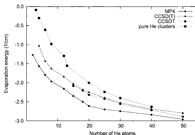
FIG. 5. Evaporation energy \Delta(n) as a function of the interaction potential and of the number of helium atoms for \text{MgHe}_n . The \Delta(n) values for pure \text{He}_n are also included. Energies in \text{cm}^{-1} .
