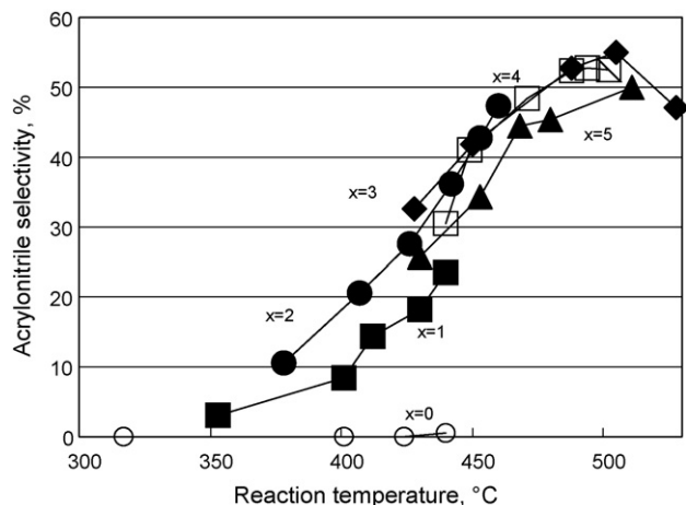
Fig. 5. Effect of reaction temperature on selectivity to acrylonitrile, for catalysts with composition Sn/V/Nb/Sb = 1/0.2/1/x.
