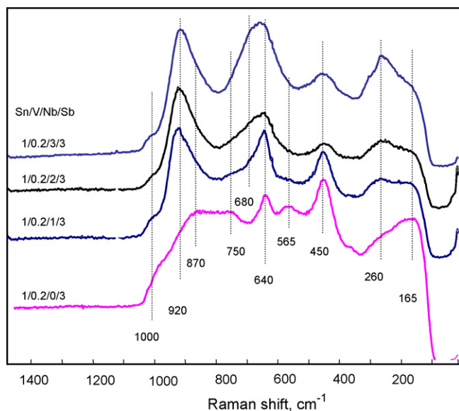
Fig. 2. Raman spectra of calcined Sn/V/Nb/Sb 1/0.2/1/ x (top) and 1/0.2/ y /3 (bottom) (atomic ratios) samples.
