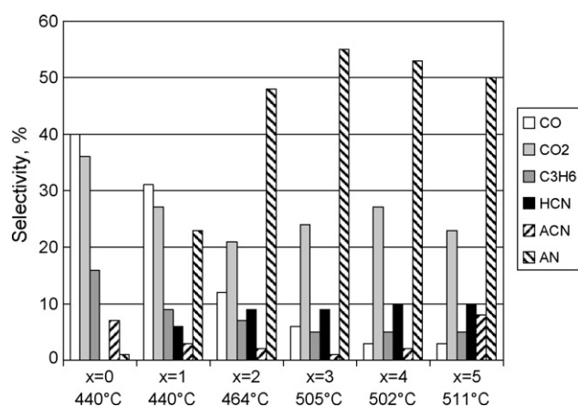
Fig. 7. Selectivity to the reaction products at the temperature at which the acrylonitrile yield is the highest, for catalysts with composition Sn/V/Nb/Sb = 1/0.2/1/x. HCN: cyanhydric acid; ACN: acetonitrile; AN: acrylonitrile.
