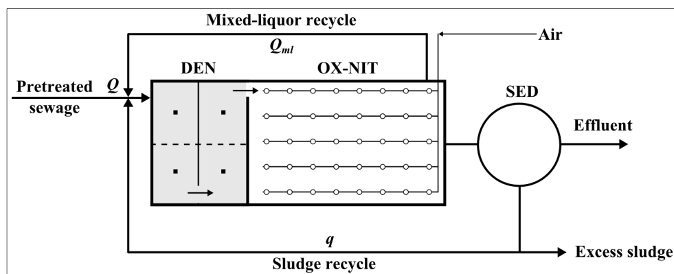
Figure 1. Pilot plant layout.
