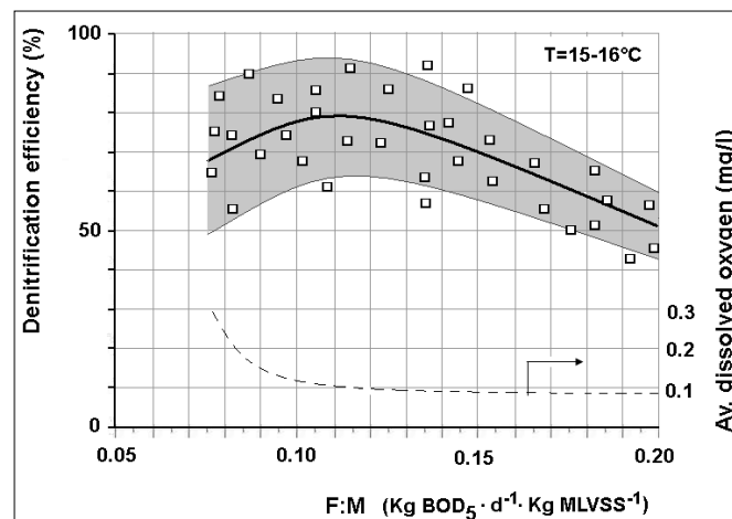
Figure 6. Efficiency of denitrification in the simultaneous process (Scheme B).
