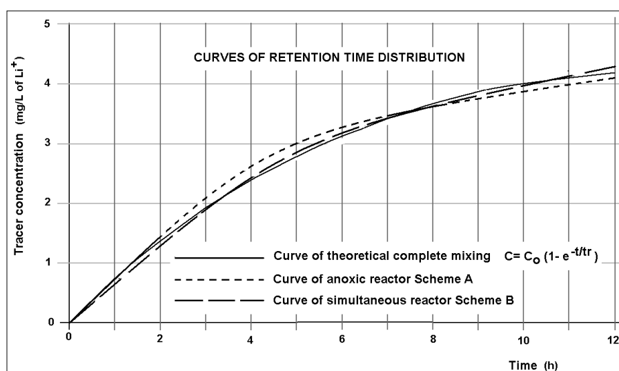
Figure 3. Retention time distribution curves of the tested units, compared with the theoretical complete-mixing curve (step dosing of 5 \text{ mg}\cdot\text{L}^{-1} of \text{Li}^+ as a tracer).
