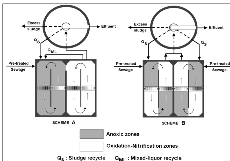
Figure 2. Alternative processes after the modifications of the base plant.
