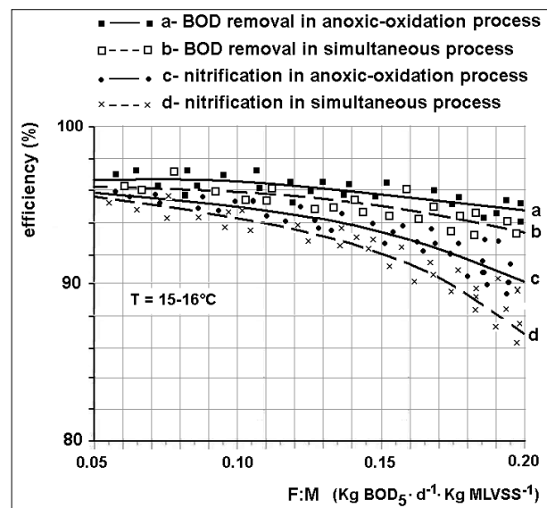
Figure 7. Efficiency of BOD_5 removal and of nitrification for the two processes studied.
