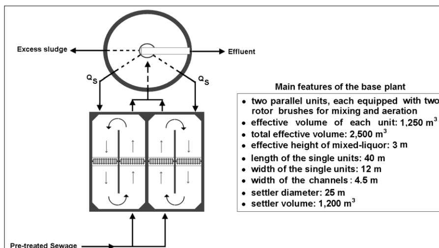
Figure 1. Modified base plant used for the tests.
