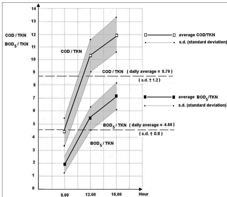
Figure 4. Trends of day-time mean COD/TKN and BOD 5 /TKN ratios in the raw sewage.
