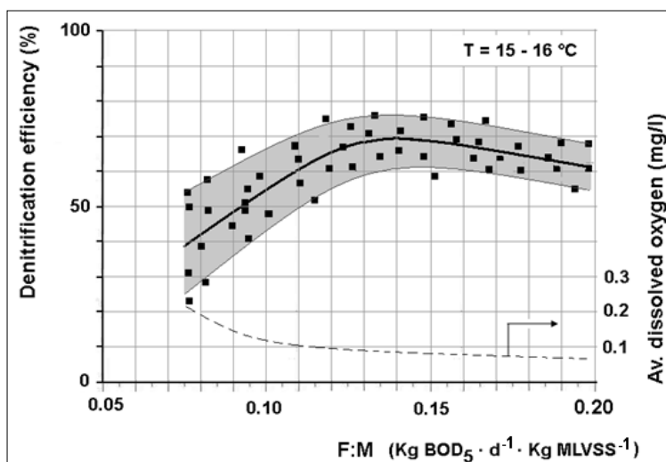
Figure 5. Efficiency of denitrification in the anoxic-aerobic process (Scheme A).
