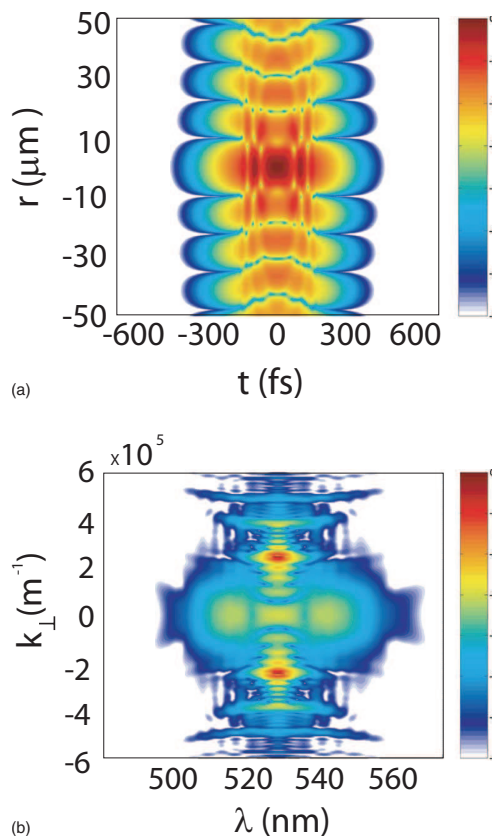
FIG. 9. (Color online) (a) Detailed near-field I(r,t) for the unsteady Bessel filament in water at propagation distance z=1.4 cm. The temporal substructures result from cyclical splitting events. (b) Angularly resolved spectra obtained from simulation of unsteady Bessel filaments at the same propagation distance.
