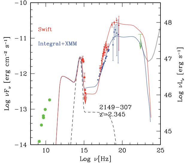
Fig. 2. Spectral Energy Distributions and models (solid lines) for Swift (red) and XMM-Newton + ISGRI (blue) data. The figure shows in green archival radio and IR data (from NED) and the EGRET upper limit (Fichtel et al. 1994). The gray line represents the GLAST sensitivity curve. The dashed line shows the input spectrum from the disk and the corona.
