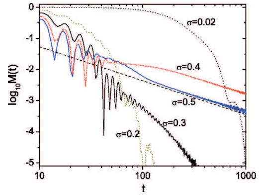
FIG. 4. (Color online) Fidelity decay for several values of \sigma with k=0.3 , N=2^{12} , \xi^2=\hbar/20 , and (\tilde{r}_0, \tilde{p}_0)=(1.2\pi, 0.28\pi) . For t around 100, the rate of fidelity decay increases for 0 < \sigma < 0.2 , then decreases for 0.2 < \sigma < 0.4 , and then increases again. This is in agreement with the semiclassical prediction that the decay rate \beta oscillates with a period |\tilde{v}'/\tilde{U}_I'| \approx 0.4 (see text). The values \tilde{U}_I' \approx 1.85 and \tilde{v}' \approx 0.76 are obtained from the classical motion. Notice that the transition time from Gaussian to power law decay of fidelity is proportional to 1/\sigma (see text). Here the power law decay is visible for \sigma=0.4 and 0.5 (the dashed straight line gives the 1/t^{1.09} decay).
