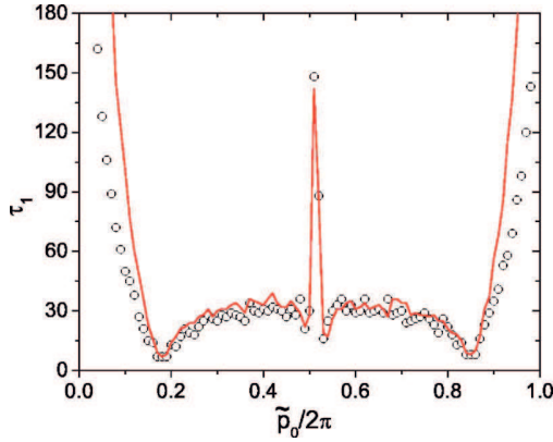
FIG. 2. (Color online) The time scale \tau_1 versus \tilde{p}_0 , for the same parameters as in Fig. 1. The circles give the values of \tau_1 calculated by the first time at which ||M(t) - M_{sc1}(t)|/M(t)| > 0.1 [see Eq. (8)]. The solid curve is the semiclassical estimate given by \sigma w_p^2 |\tilde{k}_{pp}(\tau_1)| = 1 , with \tilde{k}_{pp}(t) numerically computed in the corresponding classical system.
