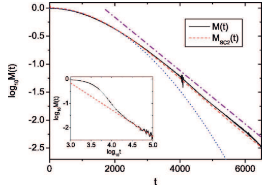
FIG. 3. (Color online) Solid curve: fidelity decay for \sigma=0.2 , N=2^{12} , k=0.3 , \xi^2 = \hbar/20 , and (\tilde{r}_0, \tilde{p}_0) = (1.2\pi, 0.8\pi) . Dashed curve: the prediction of Eq. (14) with c=1 and \tilde{U}'_1 \approx -0.019 , \tilde{U}''_1 \approx 0.042 numerically computed from the classical system. Dotted curve: the Gaussian decay e^{-(w_p \sigma \tilde{U}'_1 t)^2/2} . [For small values of \sigma , the difference between this decay and M_{sc1} in Eq. (8) is small before \tau_1 .] The dash-dotted line shows the approximate, intermediate, exponential decay. Inset: long time decay for the same case with \tilde{r}_0 = 0.6\pi (every 500 steps shown). The dashed line gives the 1/t^{1.1} decay.
