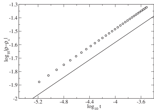
FIG. 4. Location of the coexistence curve as obtained by numerical integration of Eq. (16) as a function of the reduced “temperature” t=|r-r_c| . A linear fit gives \beta=0.33\pm 0.03 , consistent with the result from the fixed point analysis \beta\approx 0.325 (solid line).
