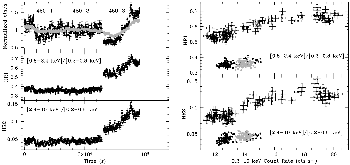
Fig. 3.—Same as Fig. 1, but for the orbit 450 observation. In the left panel, the offsets of the normalized light curves ( top ) between exposures 450-1 (medium filter), 450-2 (thin filter), and 450-3 (thick filter) are caused by the different normalization with their own mean count rates. The different filters used also result in offsets in the hardness ratios between the three exposures, as seen from the middle and bottom panels, which are particularly significant between exposures 450-2 and 450-3. In the right panel, the error bars for exposures 450-1 ( black ) and 450-2 ( gray ) are not shown for clarity, but are similar to those of exposure 450-3 ( black with error bars ). Also note that the different filters adopted give offsets in the total 0.2–10 keV count rates between the three exposures. [See the electronic edition of the Journal for a color version of this figure.]
