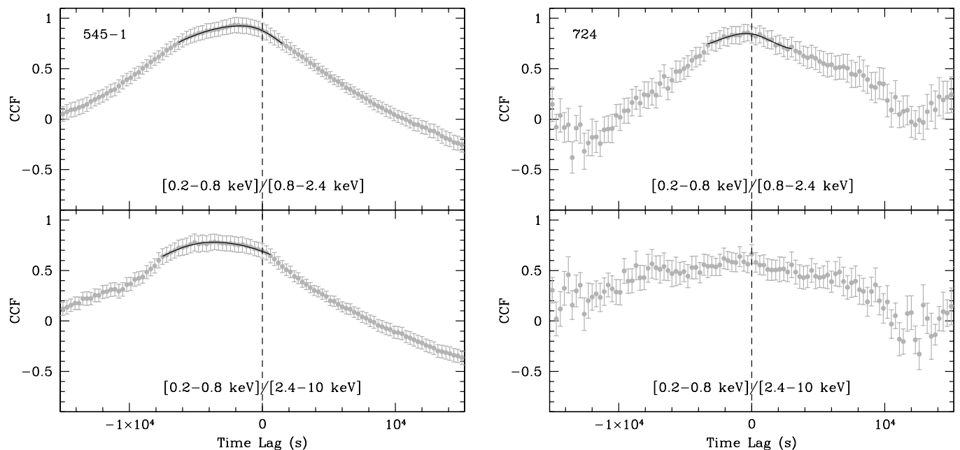
FIG. 9.—Same as Fig. 6, but for exposures 545-1 (left) and 724 (right). The lag is not measured for the soft/hard case of exposure 724, because the CCF peak is not well defined. [See the electronic edition of the Journal for a color version of this figure.]
