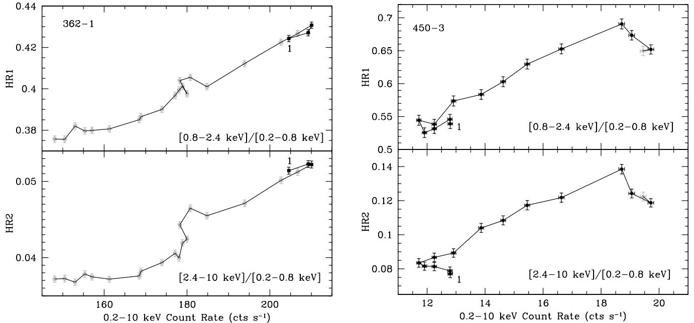
FIG. 10.—Hardness ratios as functions of the 0.2–10 keV count rates. The data are binned in 2000 s. Black points indicate the rising part of the flare, and the gray points the decaying part of the flare. The loops start from the point numbered with “1” and follow the connecting lines. The left plot is for flare 362-1, and the right plot for flare 450-3. The loops are not well defined, since both flares were not fully sampled. It appears that flare 362-1 shows an identical path, while flare 450-3 does not, for the rising and decaying phase of the flare. [See the electronic edition of the Journal for a color version of this figure.]
