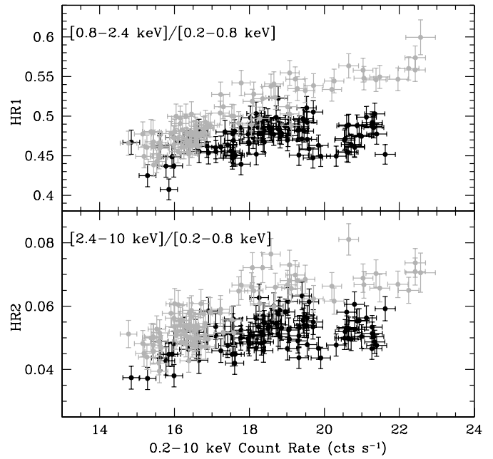
FIG. 4.—Same as Fig. 1, but for the orbit 545 observation. In the right panel, the relationships between the hardness ratios and the total 0.2–10 keV count rates are plotted with black and gray colors for the decaying and rising parts of the light curve, respectively. It is clear that the spectral variability rate is larger for the rising part than for the decaying part. [See the electronic edition of the Journal for a color version of this figure.]
