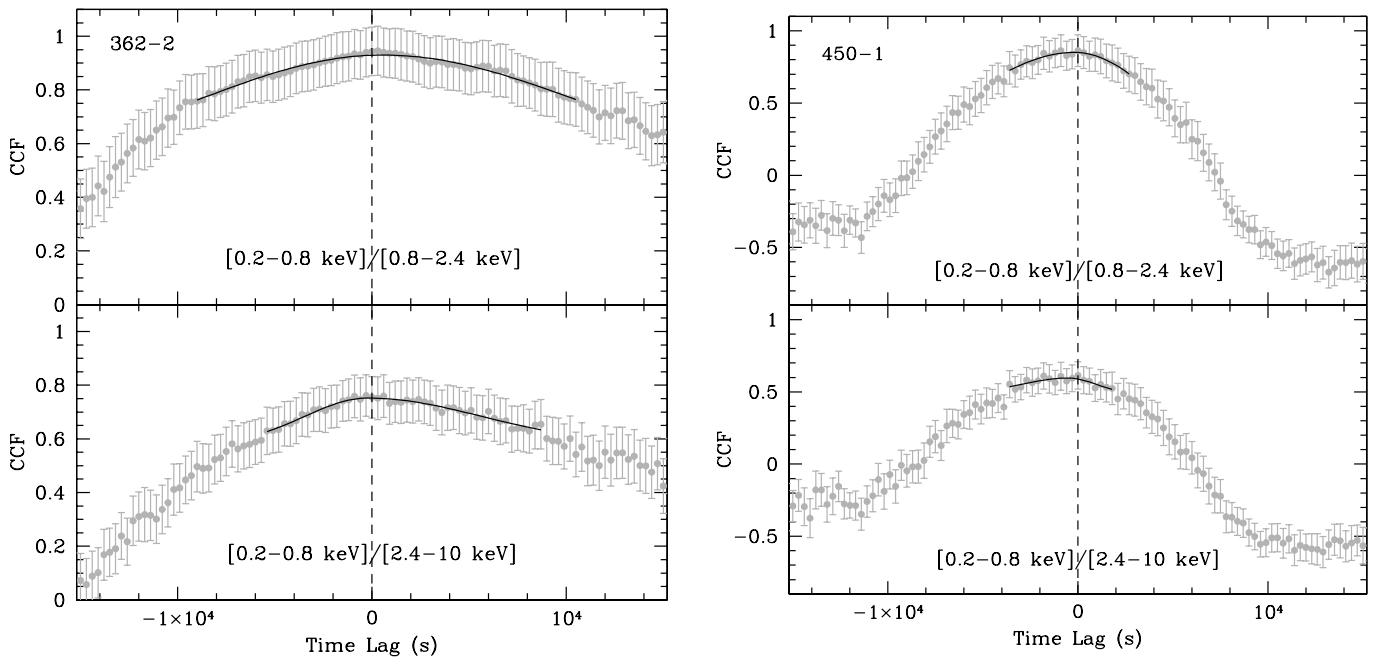
FIG. 7.—Same as Fig. 6, but for exposures 362-2 (left) and 450-1 (right). [See the electronic edition of the Journal for a color version of this figure.]
