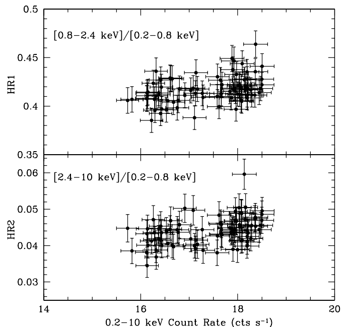
FIG. 5.—Same as Fig. 1, but for the orbit 724 observation. [See the electronic edition of the Journal for a color version of this figure.]
