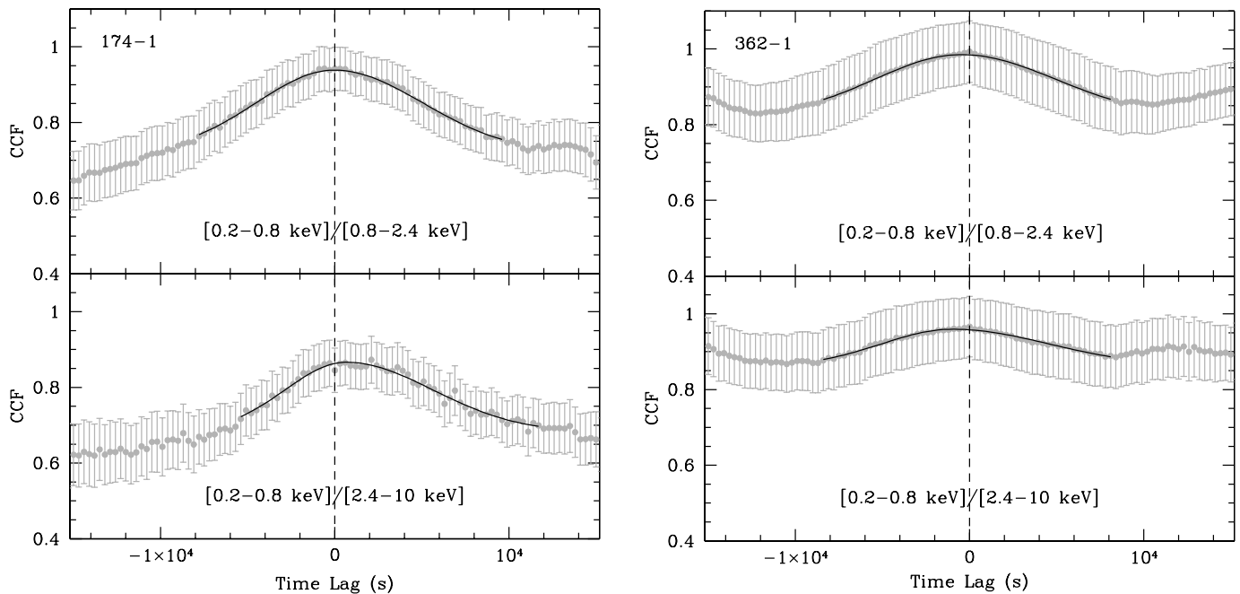
FIG. 6.—Central \pm 15 ks part of the CCF (gray points with error bars). The solid black line is the best fit with an asymmetric Gaussian function plus a constant. The left plot is for exposure 174-1, and right plot for exposure 362-1. [See the electronic edition of the Journal for a color version of this figure.]
