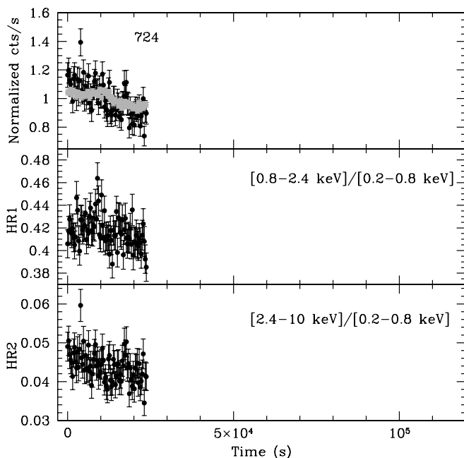
FIG. 5.—Same as Fig. 1, but for the orbit 724 observation. [See the electronic edition of the Journal for a color version of this figure.]
