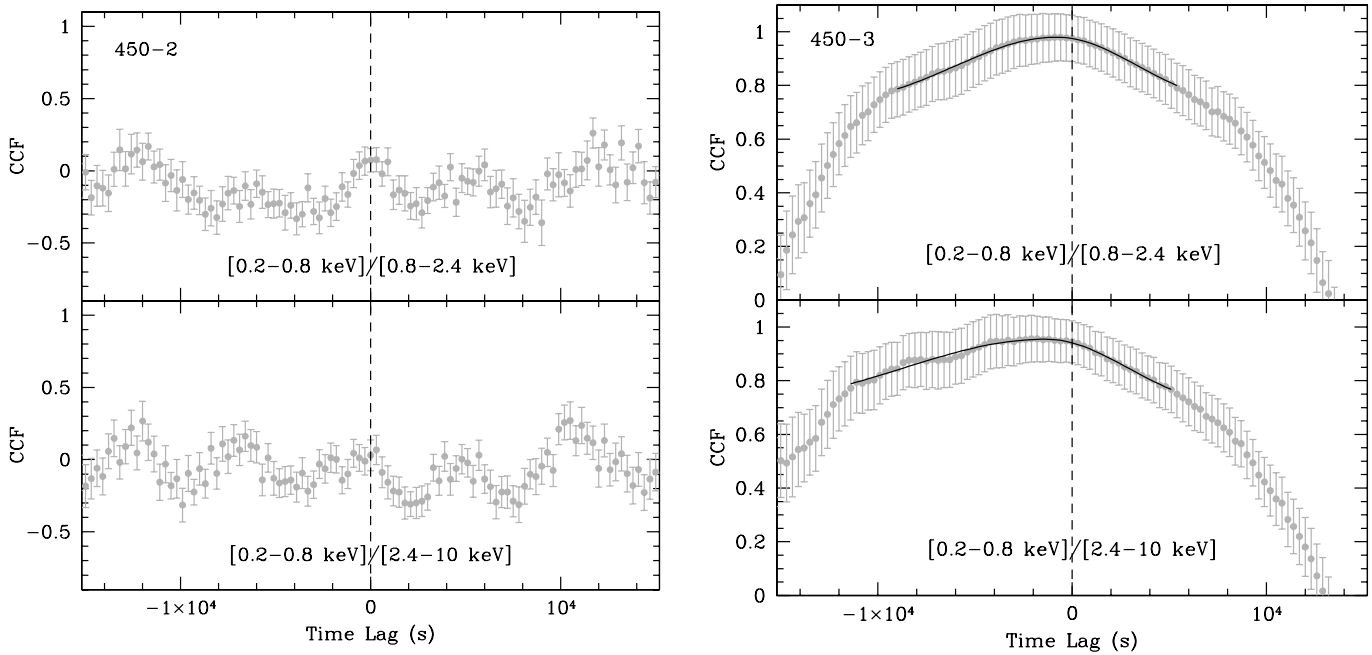
FIG. 8.—Same as Fig. 6, but for exposures 450-2 (left) and 450-3 (right). The lags are not measured for exposure 450-2, because there were no correlations. [See the electronic edition of the Journal for a color version of this figure.]
