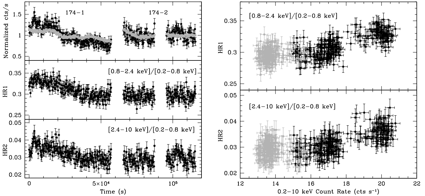
Fig. 1.—Orbit 174 observation. Left : The top panel plots the normalized 0.2–0.8 keV ( gray ) and the 2.4–10 keV ( black ) energy band light curves. The offsets of the normalized light curves between exposures 174-1 and 174-2 are caused by the different normalization with their own mean count rates. The middle and bottom panels plot the 0.8–2.4 keV/0.2–0.8 keV hardness ratios (HR1) and the 2.4–10 keV/0.2–0.8 keV hardness ratios (HR2) as functions of time, respectively. Both the light curves and hardness ratios are binned in 300 s. Right : The top and bottom panels plot HR1 and HR2 as functions of the total 0.2–10 keV count rates, respectively (exposure 174-1 is in black, and exposure 174-2 in gray). Note that the different extraction regions yield a small offset of the 0.2–10 keV count rates between the two exposures. [See the electronic edition of the Journal for a color version of this figure.]
