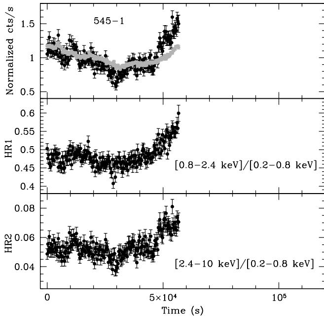
FIG. 4.—Same as Fig. 1, but for the orbit 545 observation. In the right panel, the relationships between the hardness ratios and the total 0.2–10 keV count rates are plotted with black and gray colors for the decaying and rising parts of the light curve, respectively. It is clear that the spectral variability rate is larger for the rising part than for the decaying part. [See the electronic edition of the Journal for a color version of this figure.]
