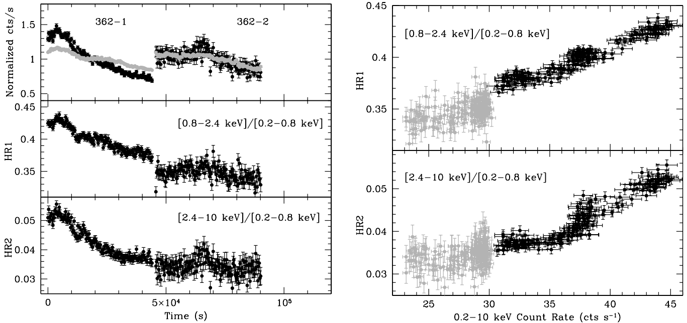
FIG. 2.—Same as Fig. 1, but for the orbit 362 observation. In the left panel, the offsets of the normalized light curves ( top ) between exposures 362-1 (in timing mode) and 362-2 (in imaging mode) resulted from the different normalization with their own mean count rates. The different operating modes also yield offsets in the hardness ratios (particularly significant in HR1) between the two exposures, as seen from the middle and bottom panels. In the right panel, the count rates of exposure 362-1 ( black ) are arbitrarily scaled down by a factor of 4.75 for smoothly connecting with those of exposure 362-2 ( gray ). [See the electronic edition of the Journal for a color version of this figure.]
