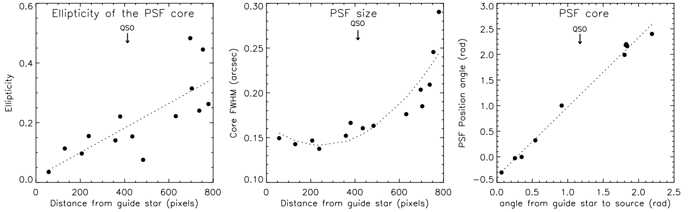
FIG. 1.—Left and middle panels show the variation of the PSF core properties with respect to the distance from the guide star. One pixel corresponds to 0.054'' . The right panel shows the relation between direction of the elongation of the PSF core and the position angle of the line connecting the star with the guide star. In all panels the position of the target is indicated with QSO.
