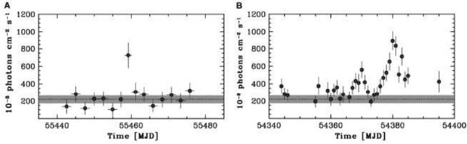
Figure 6.5 Crab Nebula light curves of the total flux detected by AGILE in the energy range 100 MeV - 5 GeV during the gamma-ray flaring periods in 2007 and 2010 (units of 10^{-8} ph \text{cm}^{-2} \text{s}^{-1} ). (Top panel:) the spinning AGILE photon flux light curve during the period September 2 - October 8, 2010. Time bins are 2.5 days except near the flare peak (2-day binning). Errors are 1\sigma . The dotted line and band marked in grey color show the average Crab flux and the 3\sigma uncertainty range. (Bottom panel:) The AGILE light curve during the period September 27 - October 12, 2007 (1-day binning) with the satellite in pointing mode. Errors are 1\sigma . The dotted line and band marked in grey color show the average Crab flux and the 3\sigma uncertainty range.
