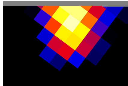
Figure 6.2 (A) Gaussian-smoothed AGILE intensity map ( \text{ph cm}^{-2} \text{s}^{-1} \text{sr}^{-1} with pixel size 0.25^\circ \times 0.25^\circ ) at E > 400 around the Vela pulsar, including only off-pulse events (i.e., discarding events with phase corresponding to Vela pulsed emission). The neutron star position is marked with a black cross; green circles are the 68% confidence contours for the position of AGL J0848–4242 and AGL J0834–4539 (Vela X). The AGILE E > 400 MeV energy band is well suited for gamma-ray imaging and provides a good compromise between the instrument-effective area ( \sim 400 \text{ cm}^2 ; \sim 100 counts from AGL J0834–4539) and PSF ( \sim 1^\circ , 68% containment radius), both parameters decreasing with energy. (B) The gamma-ray diffuse source AGL J0834–4539. AGILE contours (left) are in the range 1.4 \times 10^{-4} to 1.6 \times 10^{-4} \text{ ph cm}^{-2} \text{ s}^{-1} \text{ sr}^{-1} , with step 4 \times 10^{-6} . HESS contours (right) are from [14].
