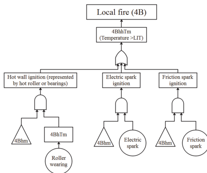
Figure 4. Fault tree for the local fire top event. 4Bhm—high mass inside node 4B; 4BhhTm—high temperature of mechanical parts inside node 4B.
