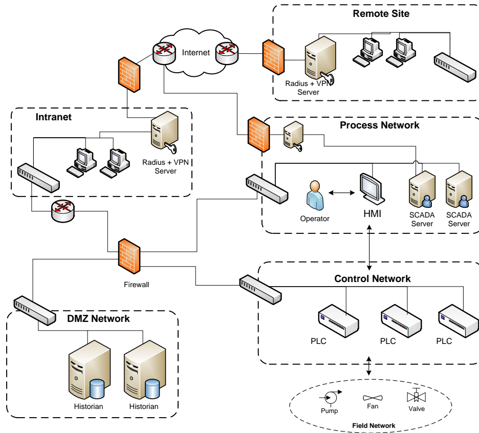
Figure 2.1: A firewalled architecture used to separate SCADA network and external networks.
