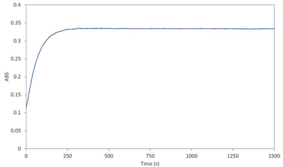
Figure 1. Absorbance vs. time of a solution of DPC and Cr(VI) at 540 nm.
