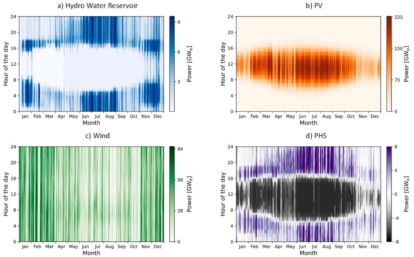
Fig. 11. Hourly power generation of hydro water reservoir (a), PV (b), wind (c) and PHS (d), with optimised HWR operation strategy, in the 2050 scenario with reference climatic year 2019.
